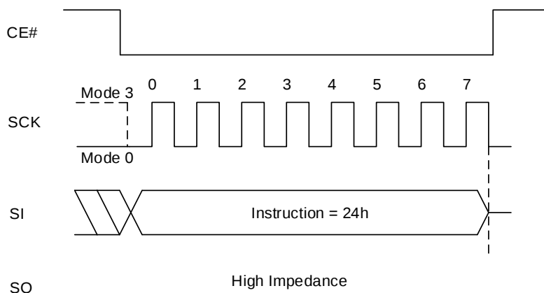
Figure 8.101 Sector Lock Sequence In SPI mode
