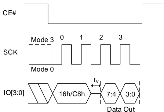
Figure 8.110 Read Bank Address Register Sequence In QPI Mode
