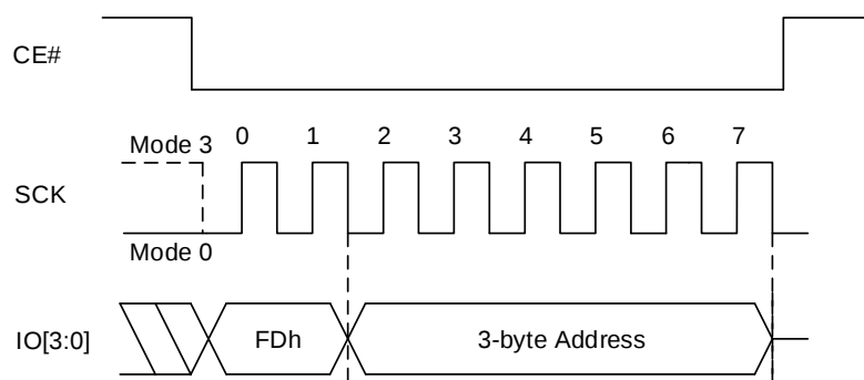
Figure 8.129 Program PPB Sequence In QPI Mode (FDh [EXTADD=0], 3-byte address)
