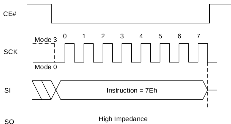
Figure 8.149 Gang Sector/Block Lock Sequence In SPI Mode
