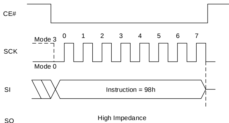
Figure 8.151 Gang Sector/Block Unlock Sequence In SPI Mode
