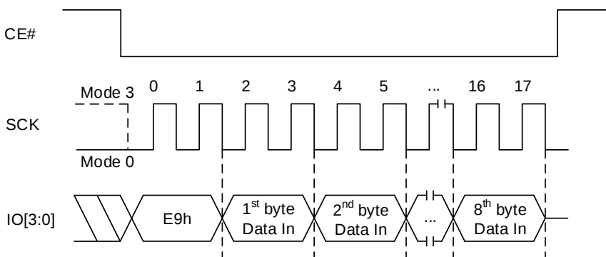
Figure 8.148 Unlock Password Sequence In QPI Mode
