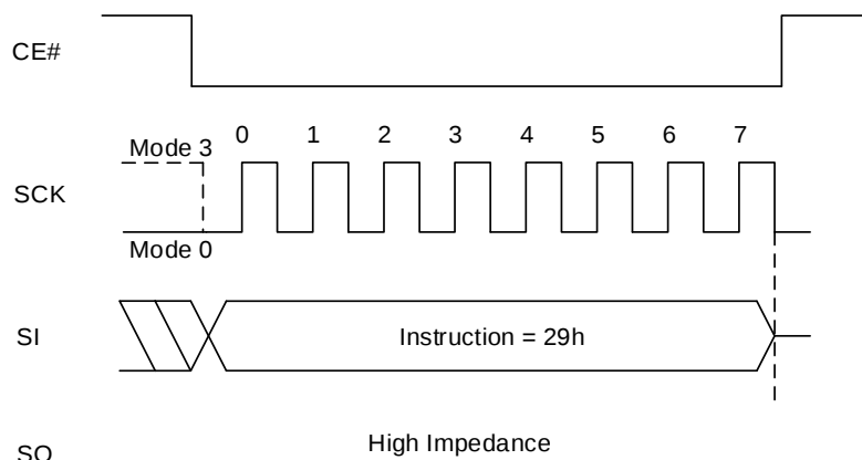
Figure 8.115 Exit 4-byte Address Mode Sequence In SPI Mode
