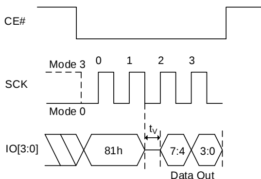
Figure 8.67 Read Extended Read Parameters Sequence In QPI Mode
