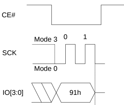
Figure 8.142 Set FREEZE Bit Sequence In QPI Mode
