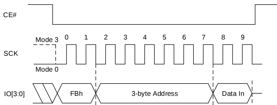
Figure 8.123 Write DYB Sequence In QPI Mode (FBh [EXTADD=0], 3-byte address)
