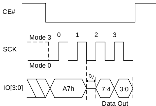
Figure 8.138 Read PPB Lock Bit Sequence In QPI Mode
