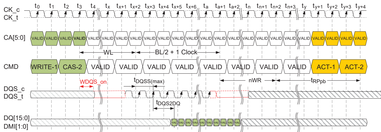
Figure 4.51 — Burst WRITE with Auto-PRECHARGE (Shown with BL16, 2tCK pre-ambles)
