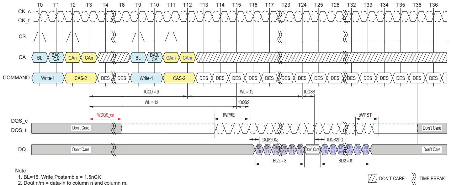
Figure 4.36 — Consecutive Writes Operation: t_{CCD} = \text{Min} + 1, 1.5nCK Postamble
