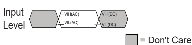
Figure 7.1a — Input Timing Definition for CKE
