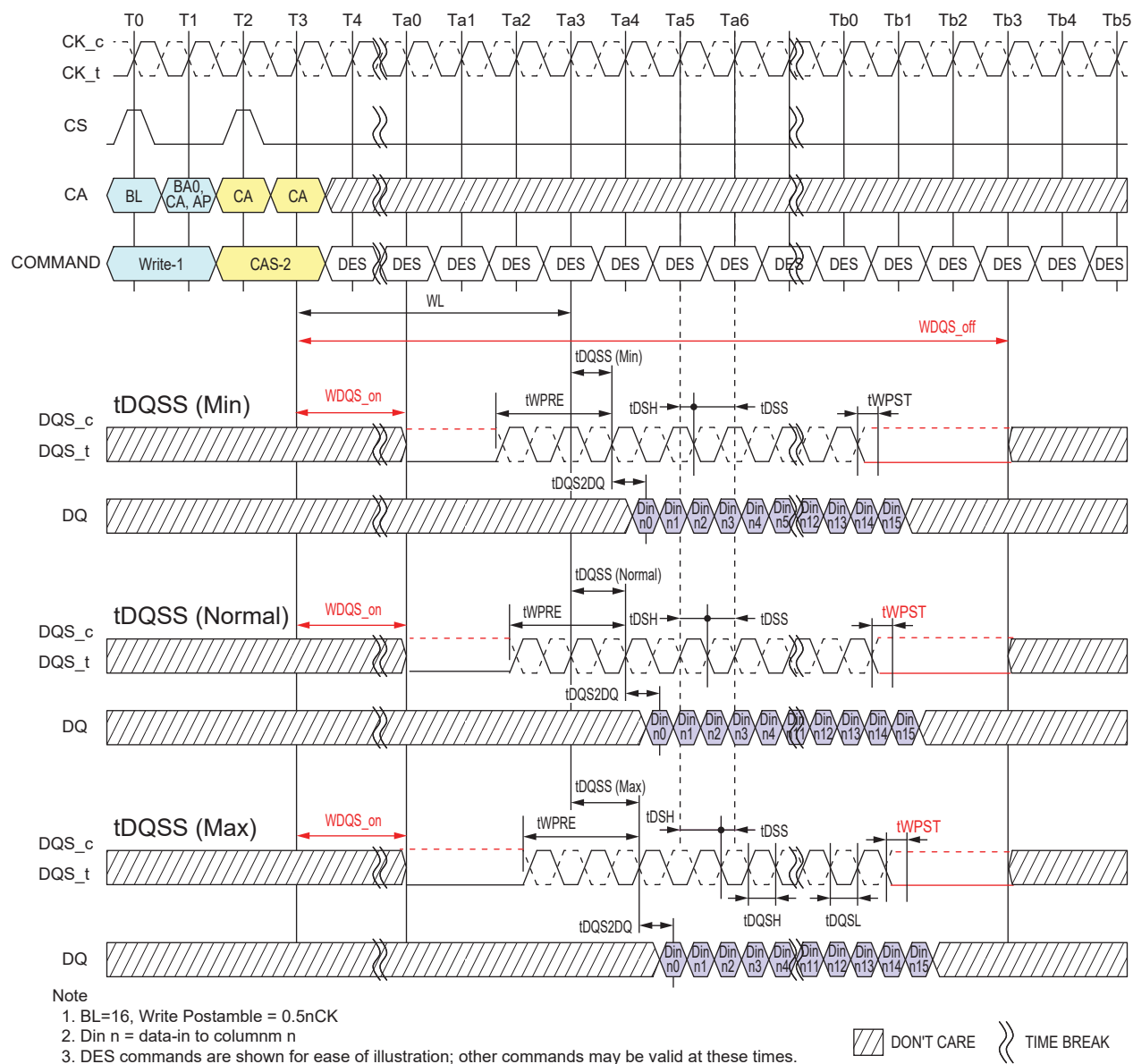
Figure 4.16 — Write Timing
