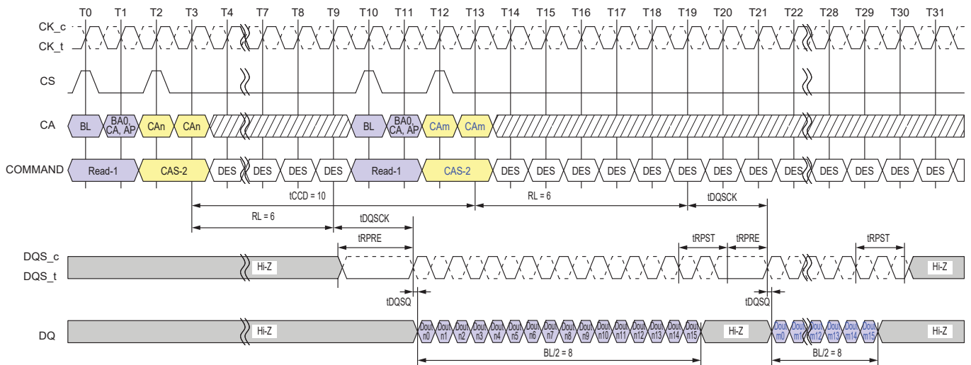
Figure 4.26 — Consecutive Reads Operation: t_{CCD} = \text{Min} + 2 , Preamble = Static, 1.5nCK Postamble
