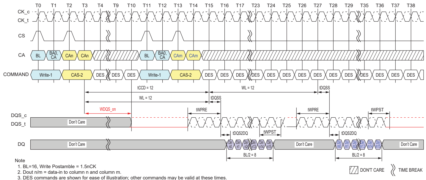
Figure 4.41 — Consecutive Writes Operation: t_{CCD} = \text{Min} + 4, 1.5nCK Postamble
