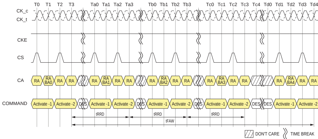
Figure 4.2 — tFAW Timing
