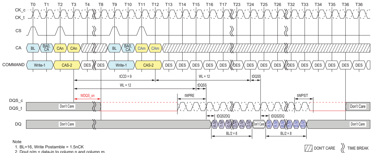
Figure 4.36 — Consecutive Writes Operation: t_{CCD} = \text{Min} + 1, 1.5n\text{CK} Postamble
