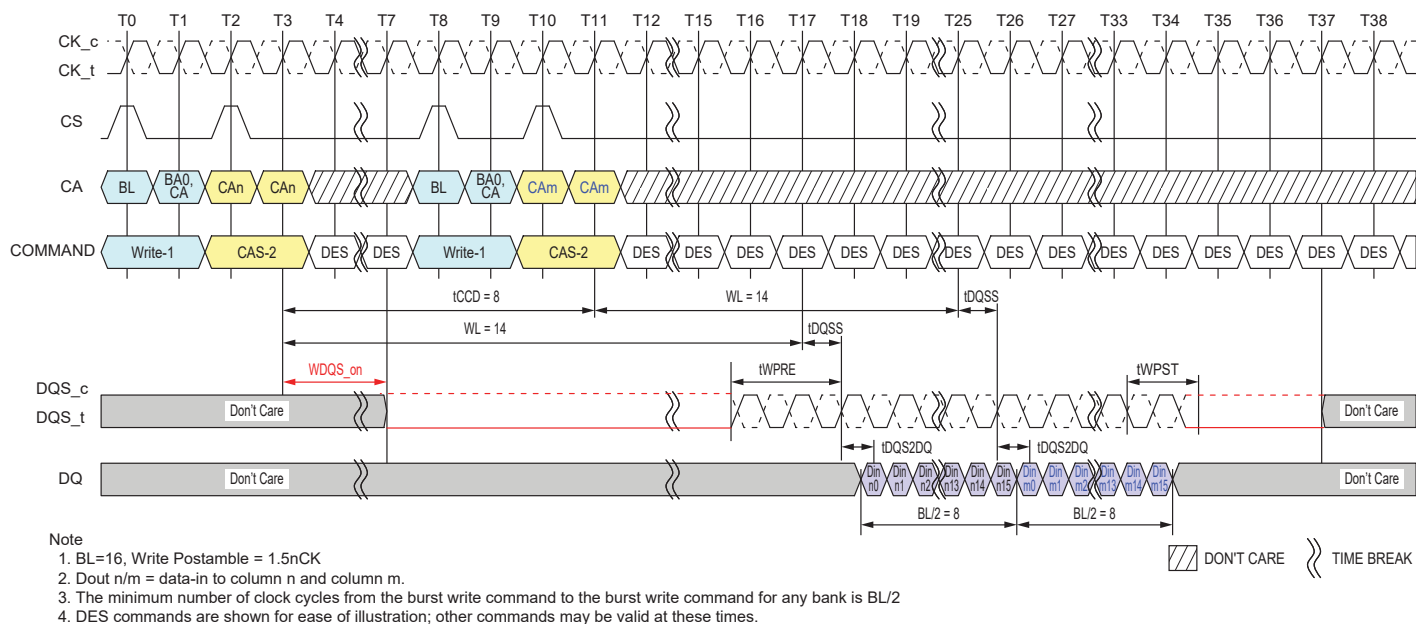
Figure 4.34 — Seamless Writes Operation: t_{CCD} = \text{Min}, 1.5nCK Postamble
