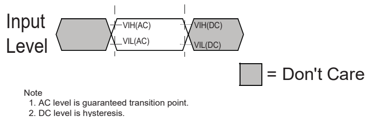
Figure 7.1a — Input Timing Definition for CKE
