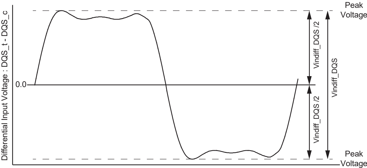
Figure 7.8 — DQS Differential Input Voltage
