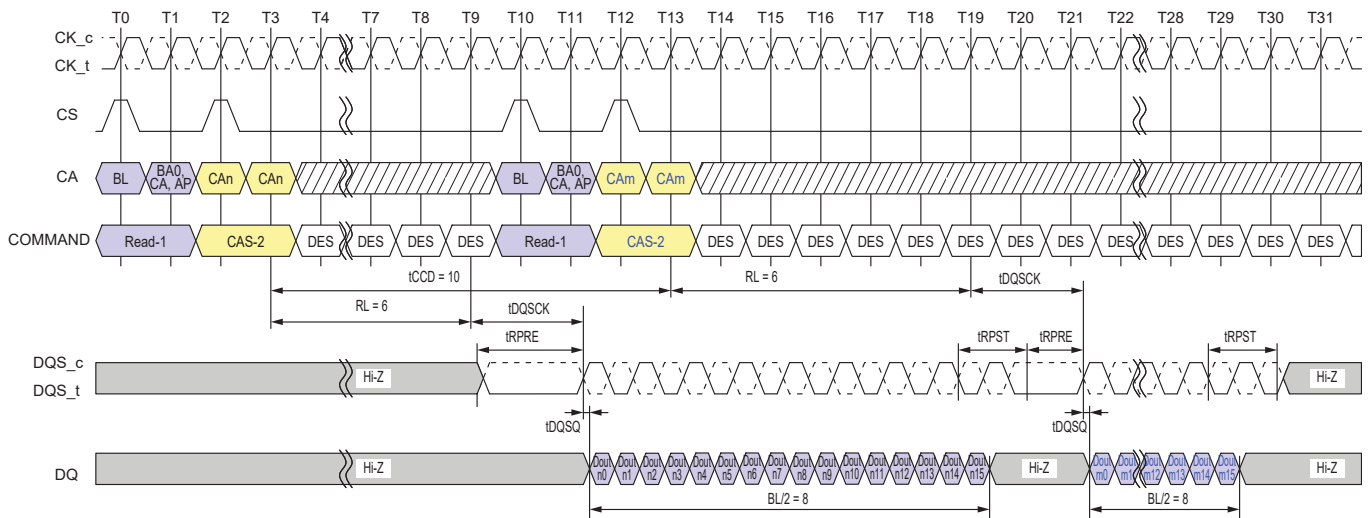
Figure 4.26 — Consecutive Reads Operation: t_{CCD} = \text{Min} + 2 , Preamble = Static, 1.5nCK Postamble
