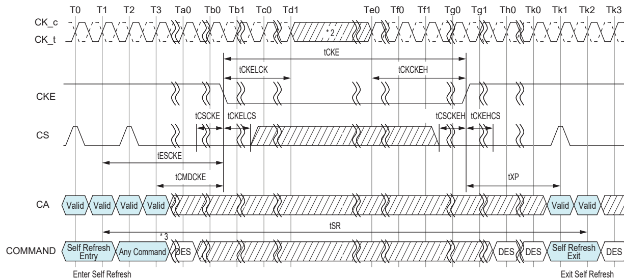
Figure 4.57 — Self Refresh Entry/Exit Timing with Power Down Entry/Exit
