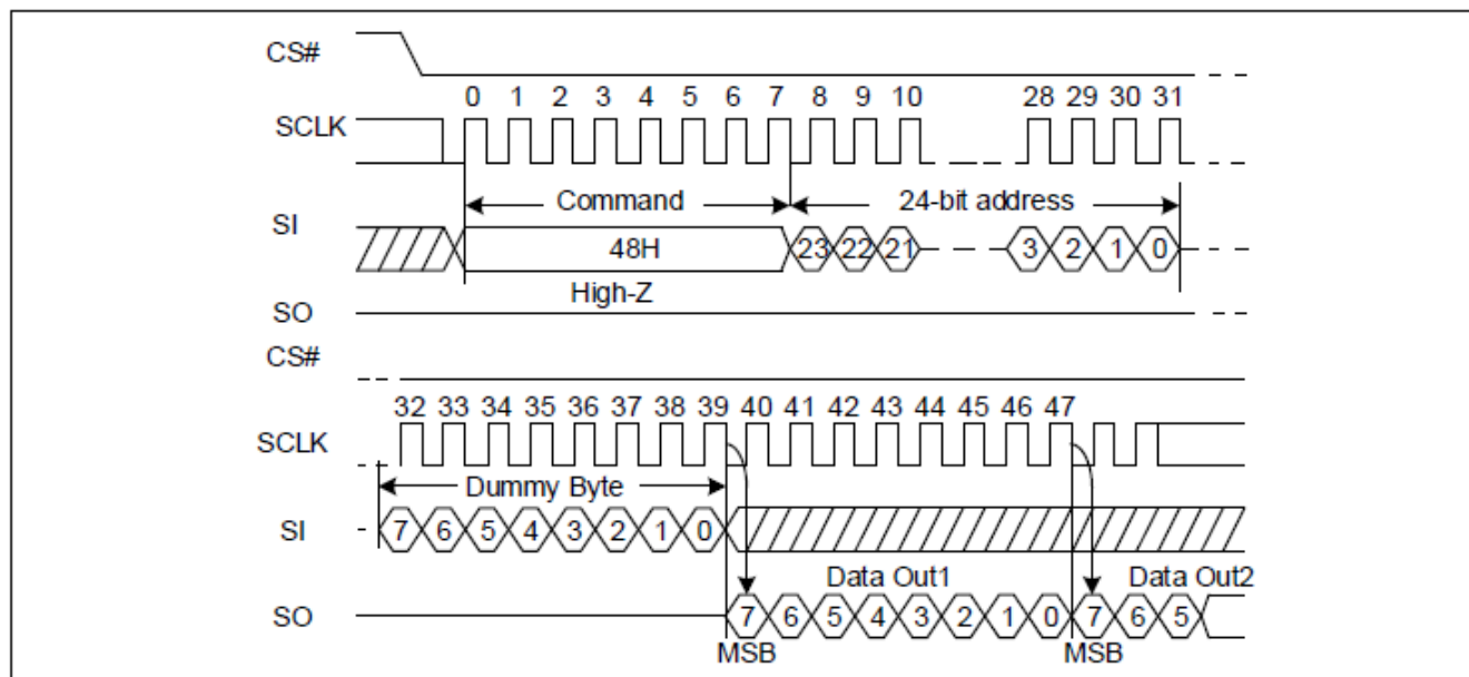
Figure 8.54 Read Information Registers Command (SPI Mode only)
