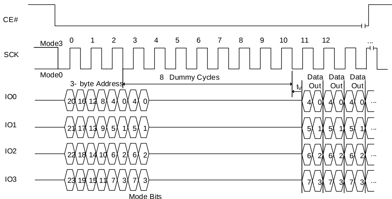
Figure 8.60 FRQDTR Sequence 2X Mode (without command decode cycles)
