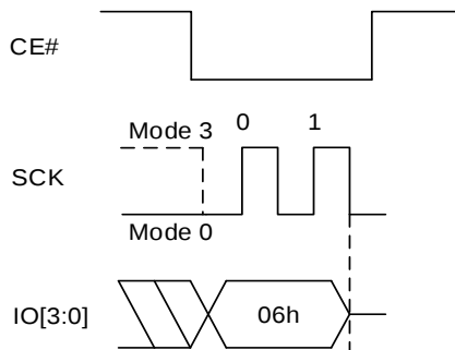
Figure 8.26 Write Enable Sequence In QPI Mode
