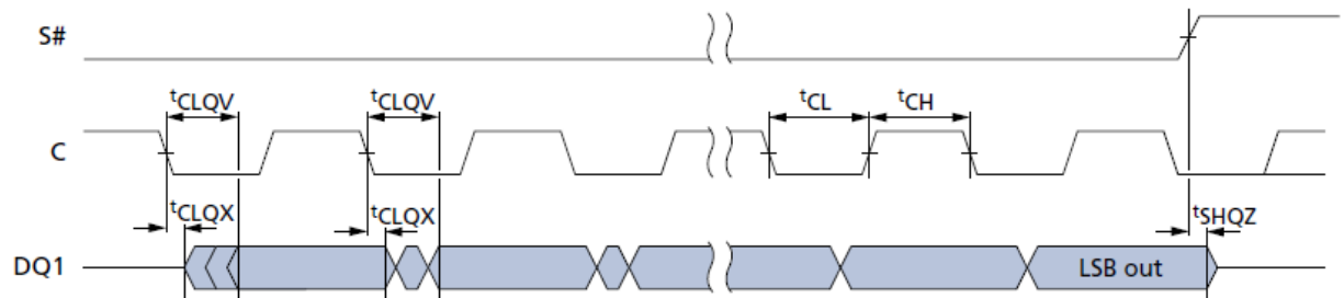
Figure 9.6 Output Timing - SDR
