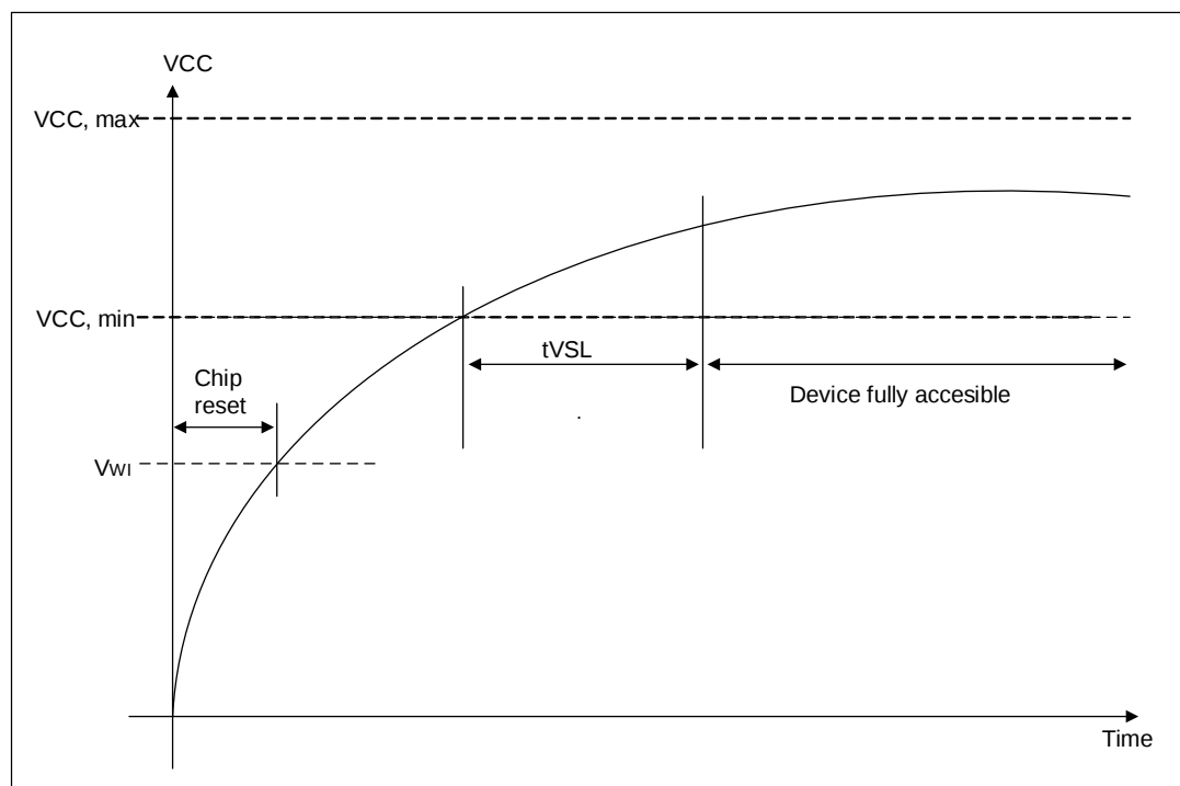
Figure 8.26 Power-Up Timing
