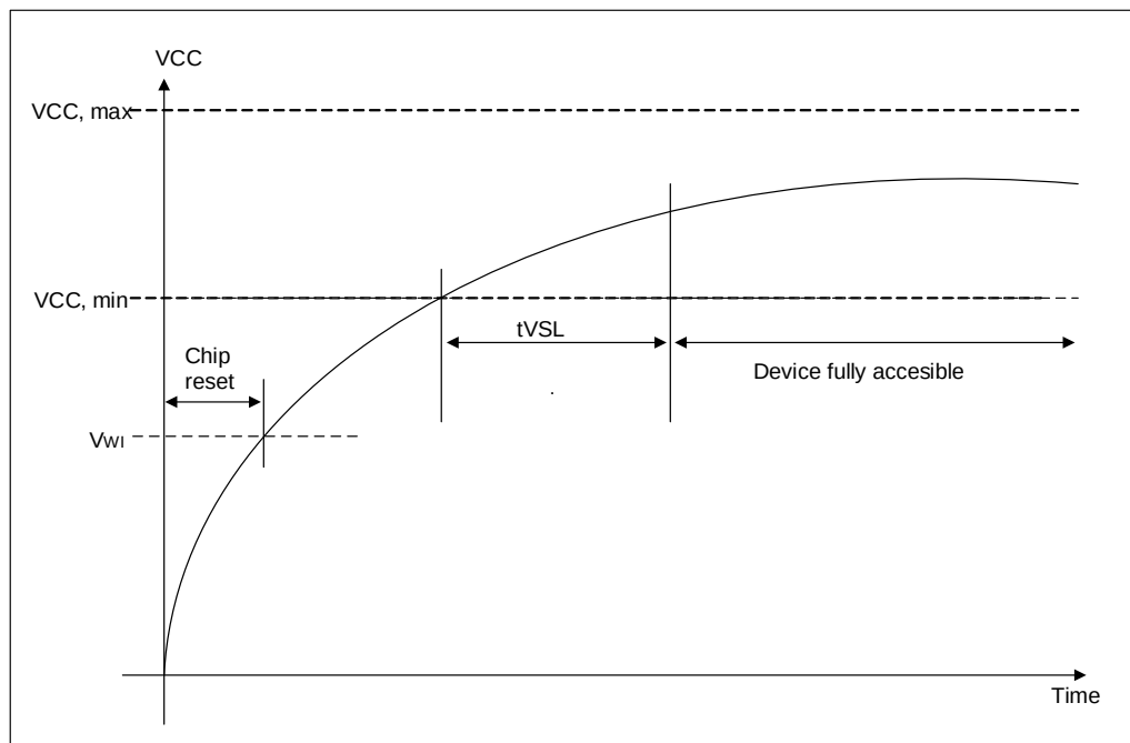
Figure 8.26 Power-Up Timing
