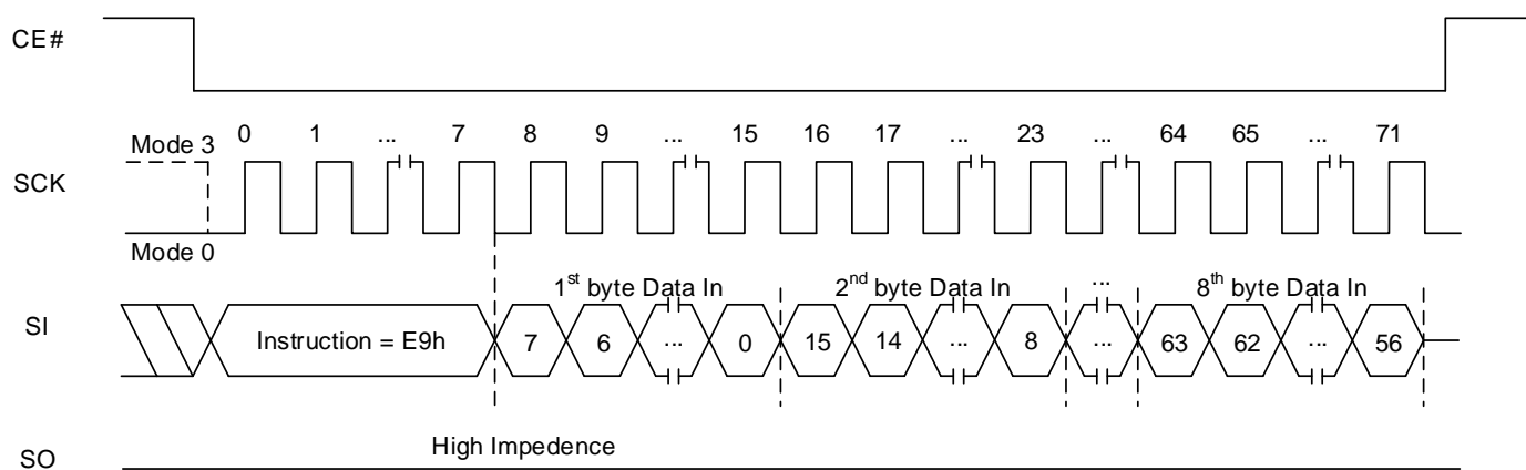
Figure 8.141 Unlock Password Sequence In SPI Mode
