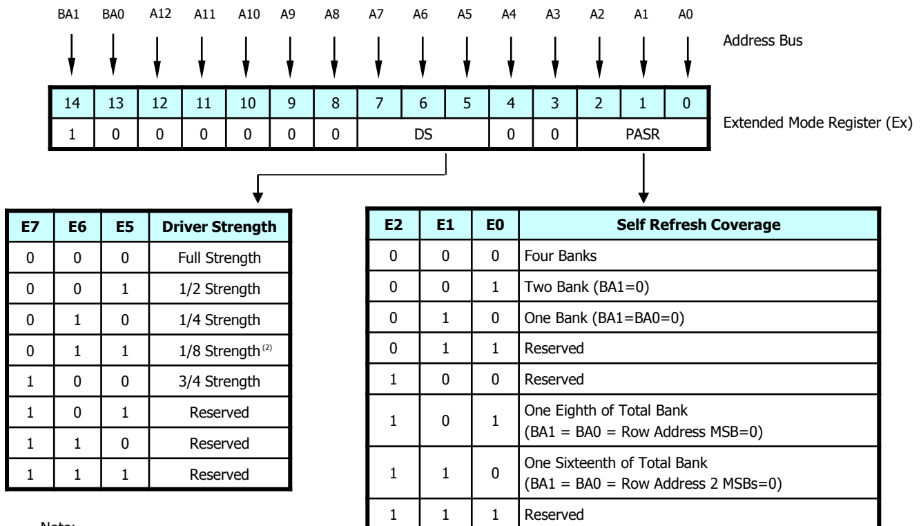
Figure 5.b : Extended Mode Set (EMRS) Register for x32
