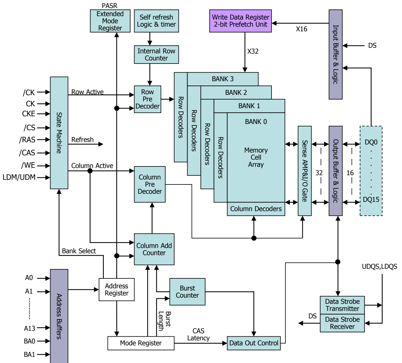
Figure 2.1 : Functional Block Diagram (64Mb X 16)
