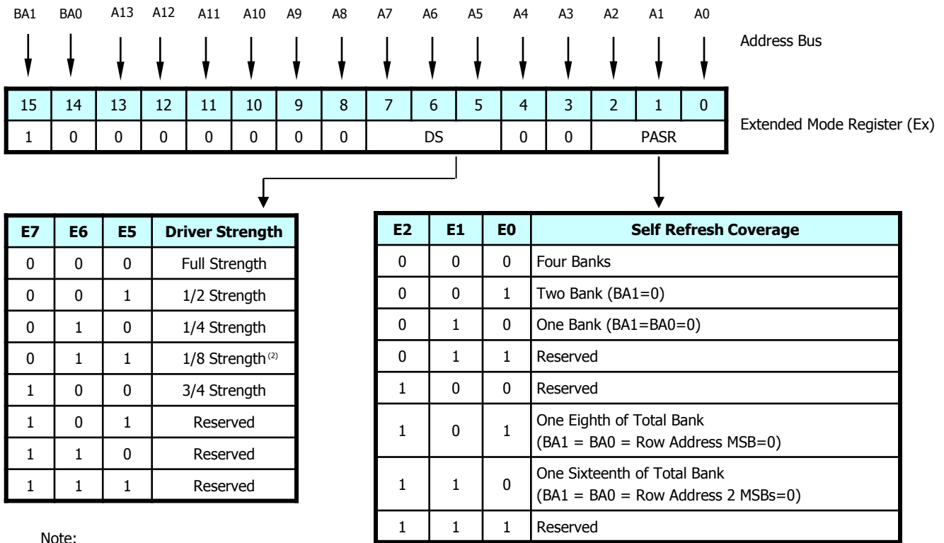
Figure 5.a : Extended Mode Set (EMRS) Register for x16
