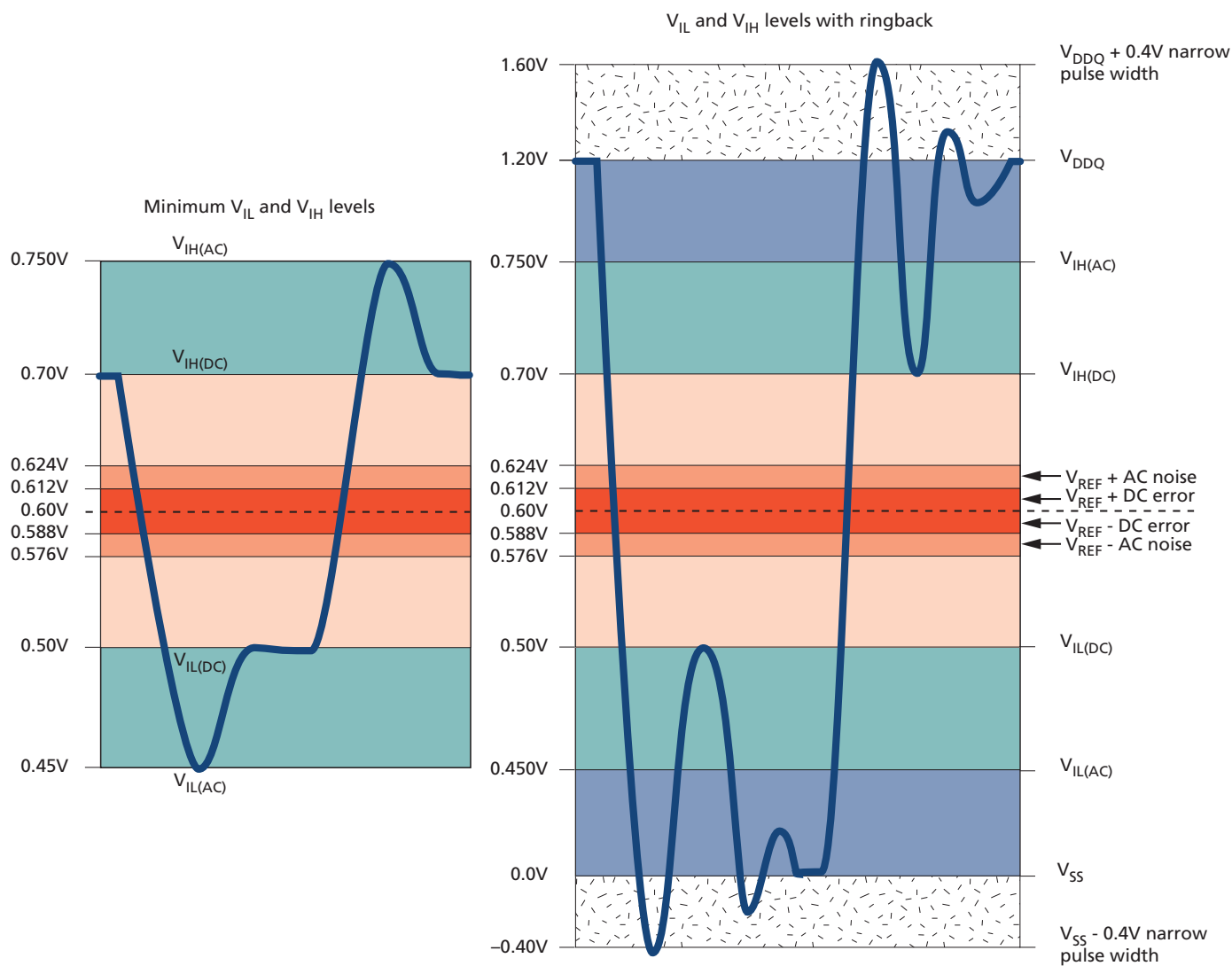
Figure 5: Single-Ended Input Signal
