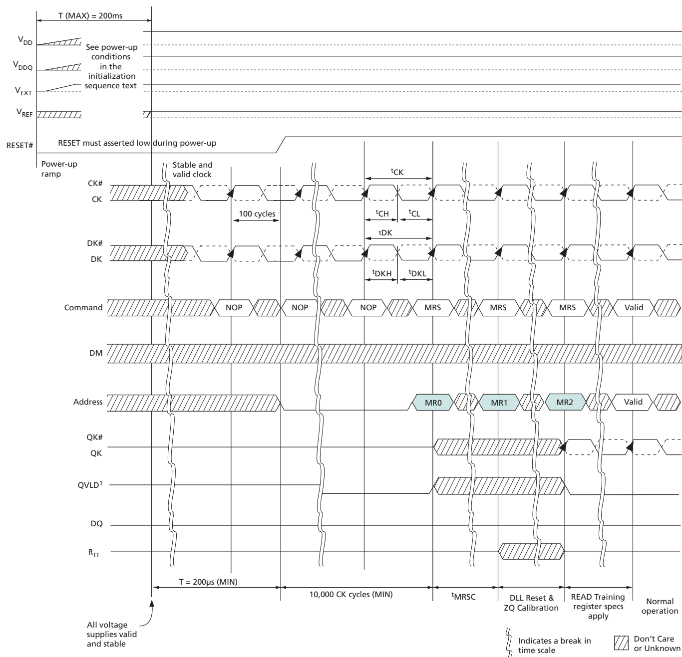
Figure 42: Power-Up/Initialization Sequence
