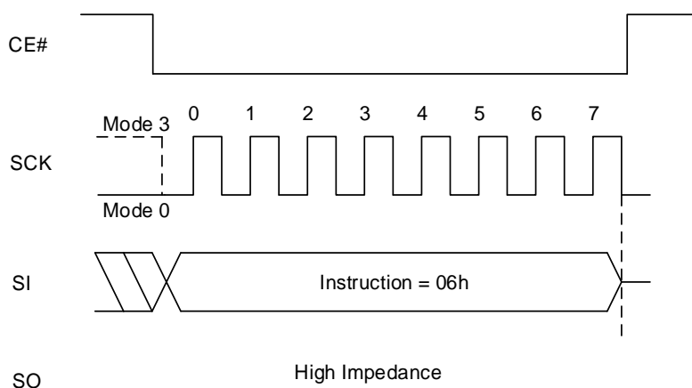
Figure 8.22 Write Enable Sequence In SPI Mode
