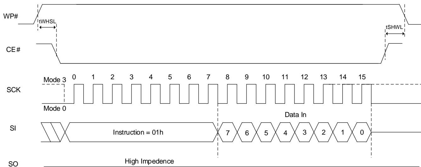
Figure 9.4 WRITE PROTECT SETUP AND HOLD TIMING DURING WRITE STATUS REGISTER (SRWD=1)
