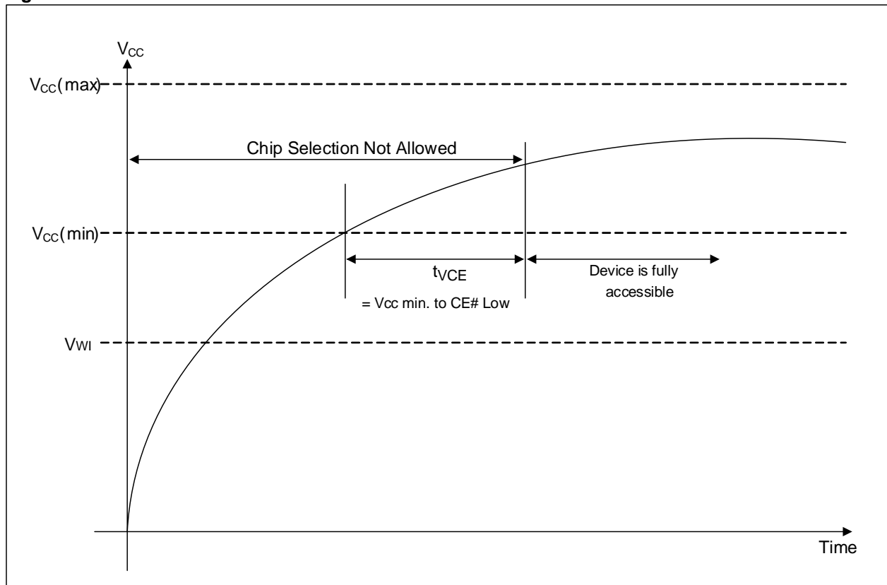
Figure 9.4 POWER UP TIMING
