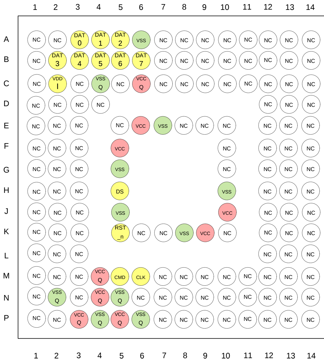
153 FBGA Top View (Ball Down)
