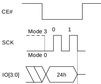
Figure 8.73 Sector Lock Sequence In QPI Mode
