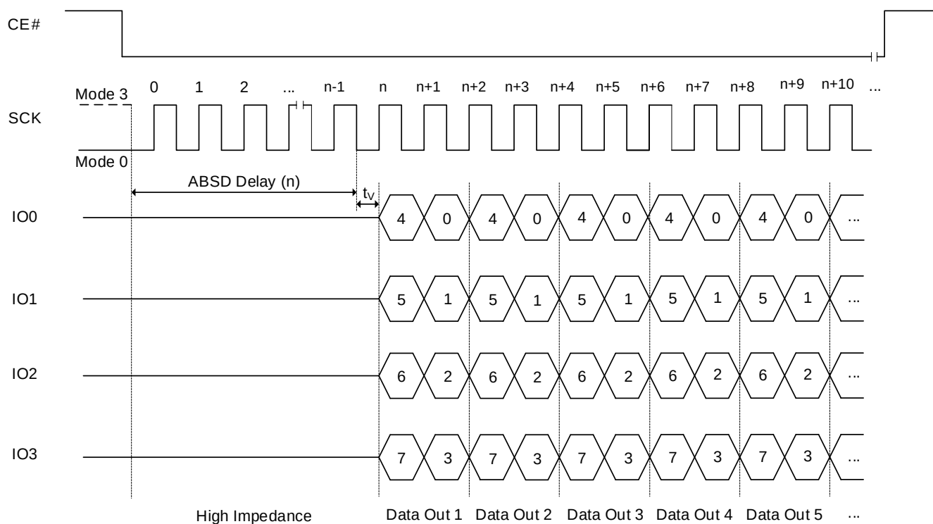
Figure 8.75 AutoBoot Sequence (QE = 1)
