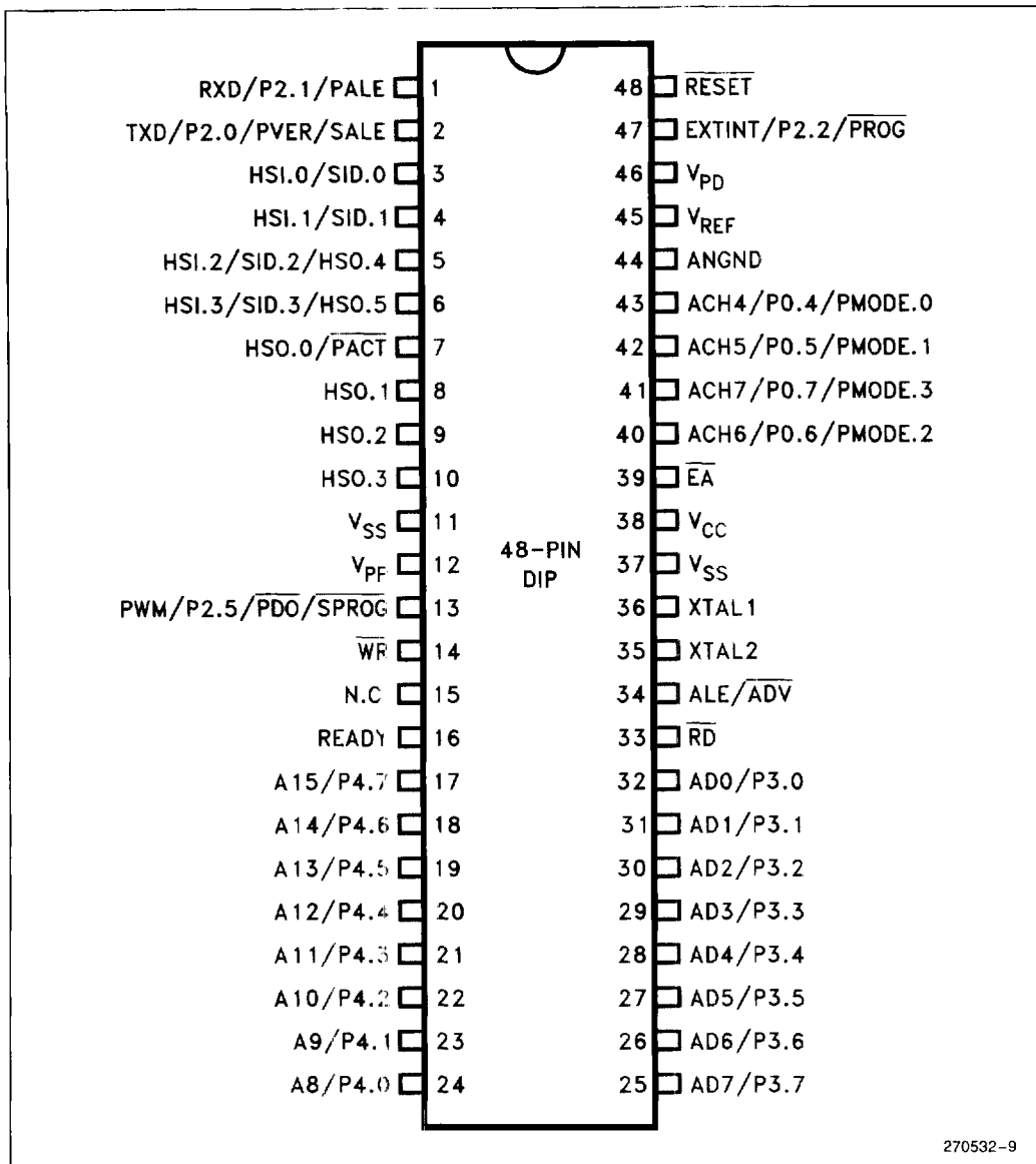
Figure 5. 48-Pin Package
