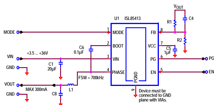
FIGURE 1. TYPICAL APPLICATION
