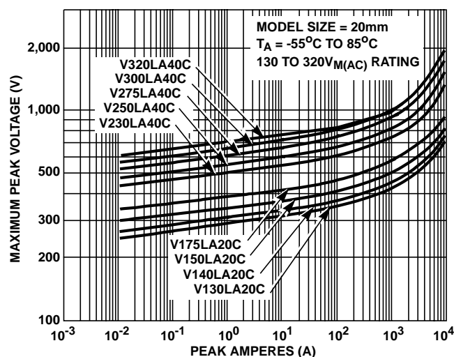
FIGURE 4. MAXIMUM CLAMPING VOLTAGE FOR V130LA20C TO V320LA40C
