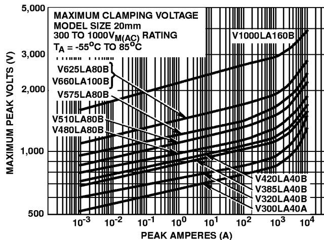
FIGURE 13. CLAMPING VOLTAGE FOR V300LA40A - V1000LA160B
