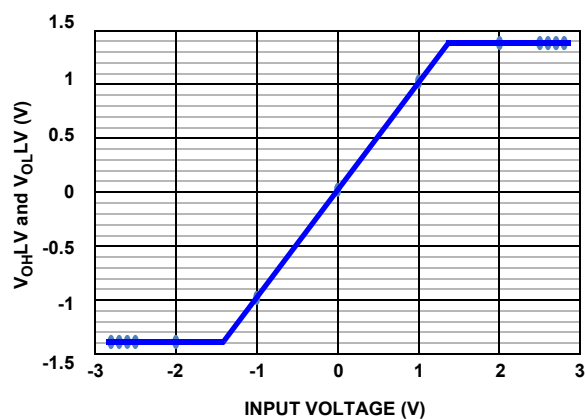
FIGURE 25. V_{OH} AND V_{OL}
