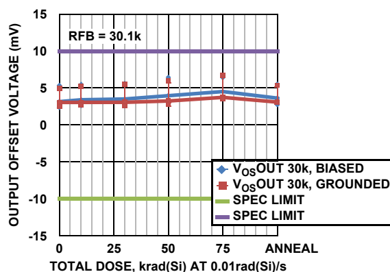
FIGURE 14. V_{OSOUT} (GAIN = 1) vs TOTAL DOSE
