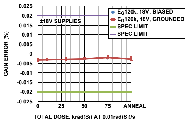
FIGURE 11. GAIN ERROR (GAIN = 1) vs TOTAL DOSE
