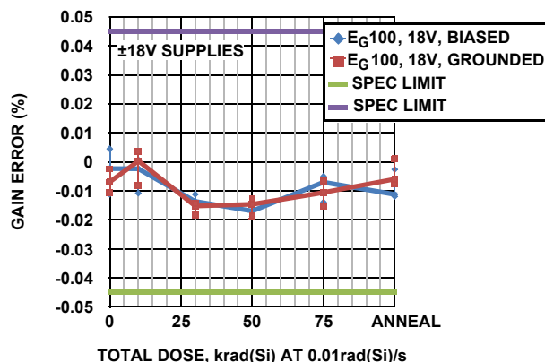
FIGURE 12. GAIN ERROR (GAIN = 100) vs TOTAL DOSE
