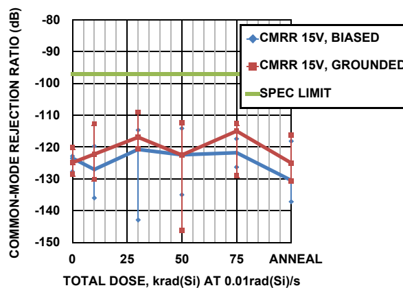
FIGURE 8. CMRR (RTI), GAIN = 100 vs TOTAL DOSE
