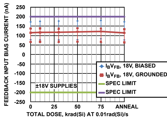
FIGURE 10. I_{BV_{FB}} vs TOTAL DOSE
