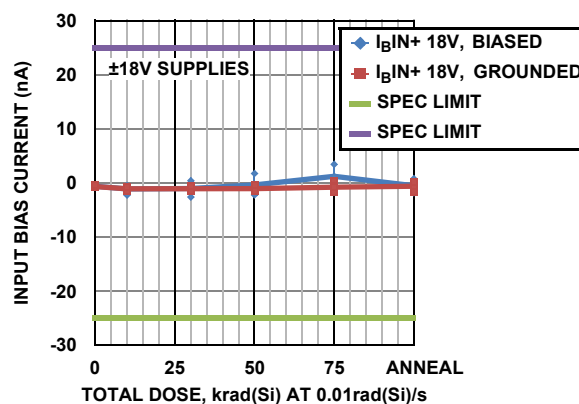
FIGURE 4. INPUT BIAS CURRENT I_{BIN+} vs TOTAL DOSE
