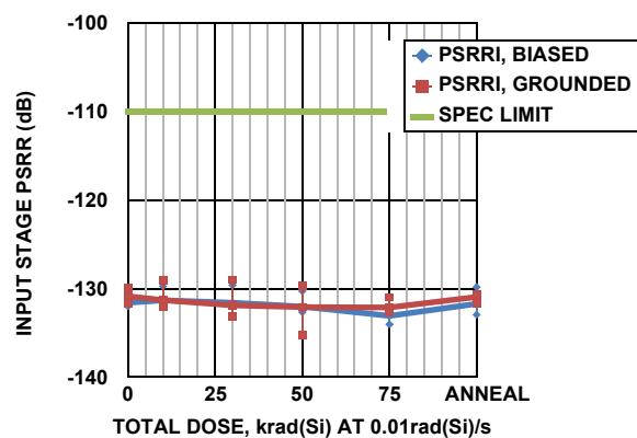
FIGURE 16. INPUT STAGE PSRR vs TOTAL DOSE
