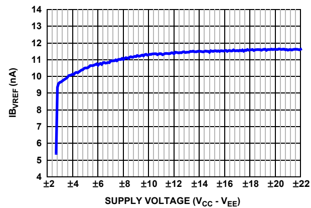
FIGURE 23. I_{BVREF} vs SUPPLY VOLTAGE ( V_{CC} - V_{EE} )
