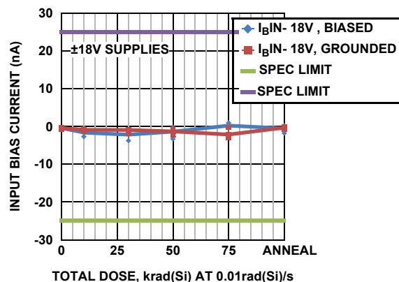
FIGURE 5. INPUT BIAS CURRENT I_{BIN-} vs TOTAL DOSE
