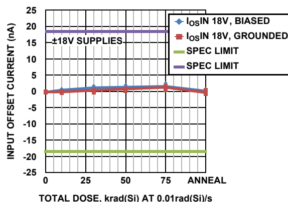
FIGURE 6. INPUT OFFSET CURRENT vs TOTAL DOSE
