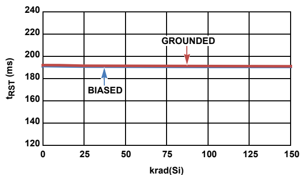
FIGURE 20. ISL705xEH t_{RST} vs LOW DOSE RATE RADIATION
