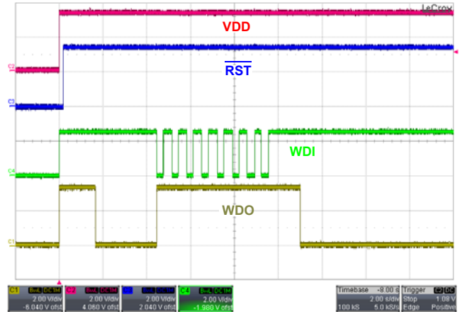
FIGURE 13. ISL706xEH START-UP TO RESET, WDO AND WDI FUNCTION
