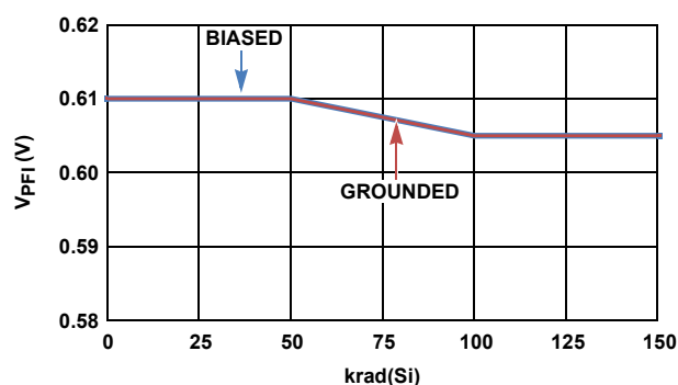
FIGURE 32. ISL706xEH V_{PFI} vs LOW DOSE RATE RADIATION
