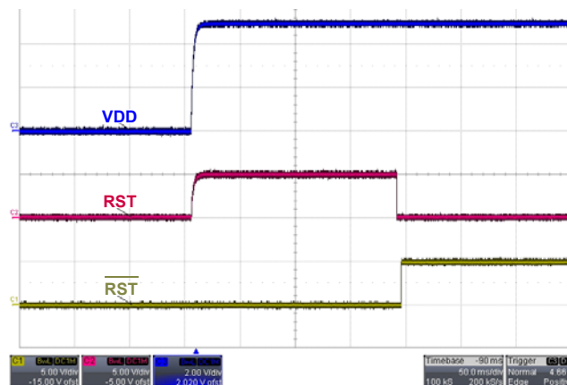
FIGURE 9. ISL705xRH RESET and \overline{RST} ASSERTION
