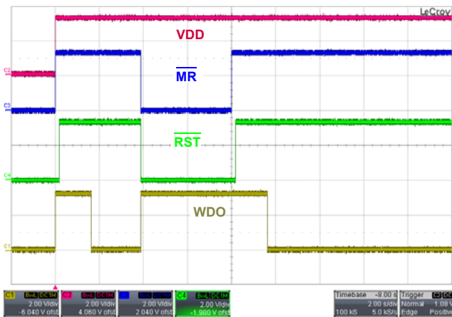
FIGURE 14. ISL706xEH START-UP TO RESET, MANUAL RESET AND WDO FUNCTION
