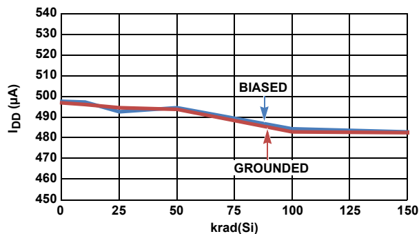
FIGURE 17. ISL705xEH I_{DD} vs LOW DOSE RATE RADIATION
