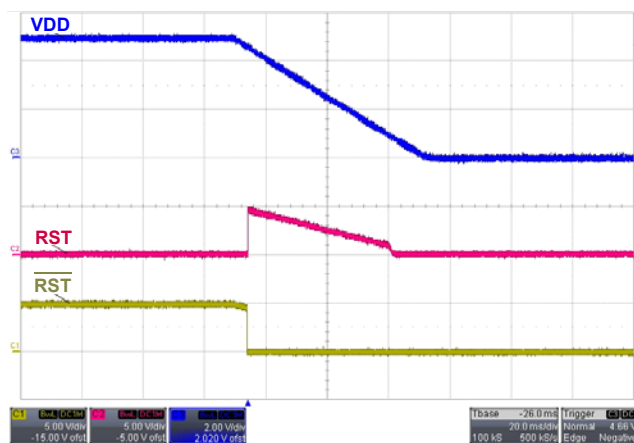
FIGURE 10. ISL705xRH RESET and \overline{RST} DEASSERTION
