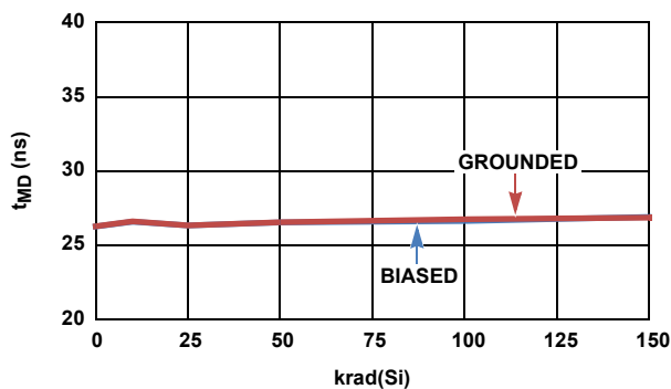
FIGURE 22. ISL705xEH t_{MD} vs LOW DOSE RATE RADIATION
