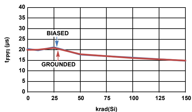
FIGURE 25. ISL705xEH t_{FPF1} vs LOW DOSE RATE RADIATION
