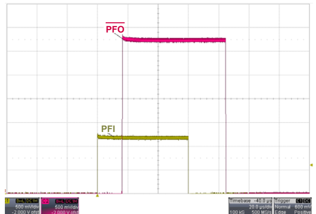
FIGURE 15. ISL705xRH PFI TO PFO RESPONSE
