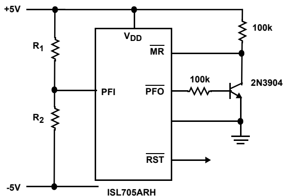
FIGURE 37. ±5V MONITORING
