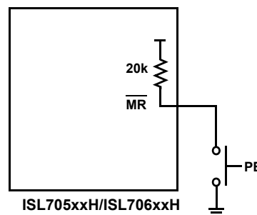
FIGURE 36. CONNECTING A MANUAL RESET PUSH-BUTTON
