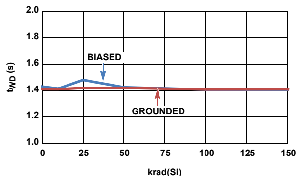
FIGURE 30. ISL706xEH t_{WD} vs LOW DOSE RATE RADIATION
