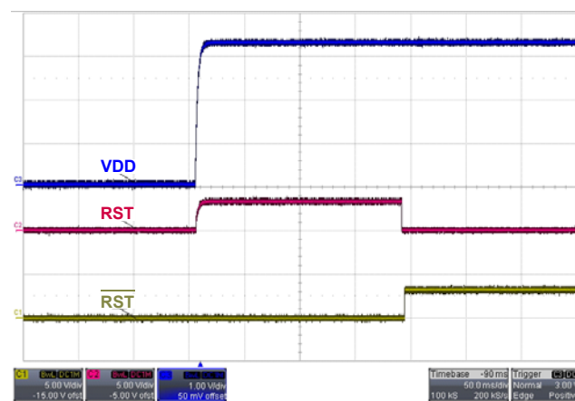
FIGURE 11. ISL706xRH RESET and \overline{RST} ASSERTION
