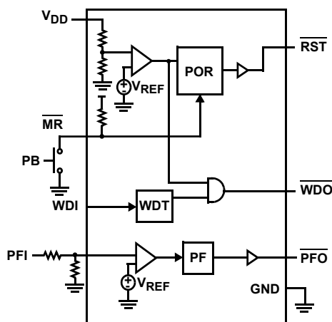
FIGURE 3A. ISL705AxH, ISL706AxH
