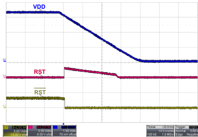
FIGURE 12. ISL706xRH RESET AND RESET DEASSERTION
