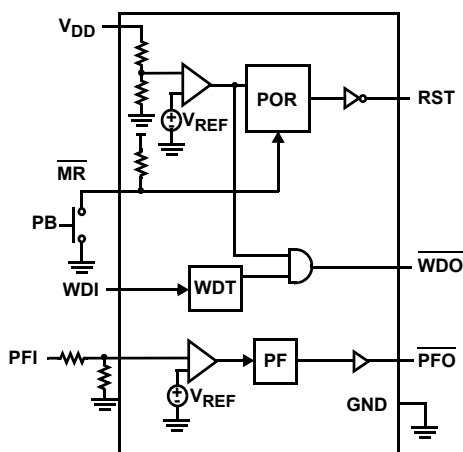
FIGURE 3B. ISL705BxH, ISL706BxH
