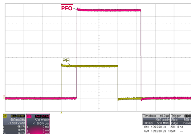
FIGURE 16. ISL706xRH PFI TO PFO RESPONSE
