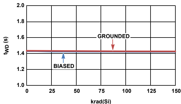
FIGURE 21. ISL705xEH t_{WD} vs LOW DOSE RATE RADIATION
