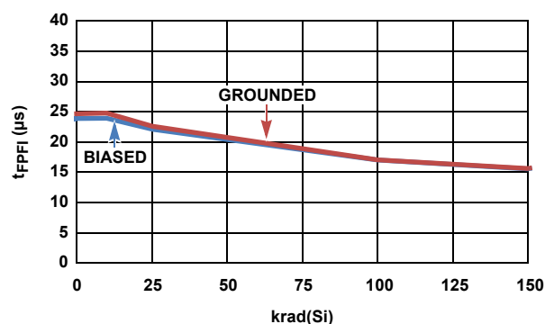
FIGURE 34. ISL706xEH t_{FPFI} vs LOW DOSE RATE RADIATION
