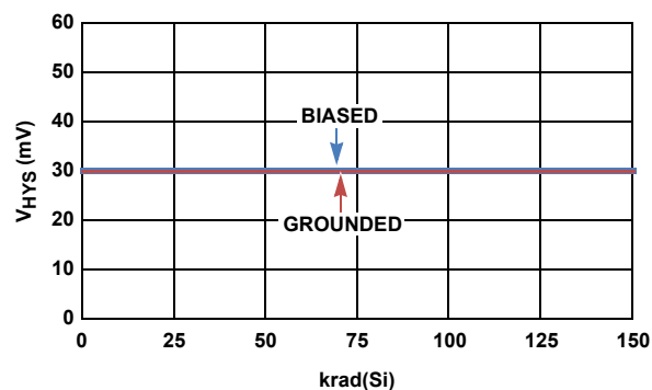
FIGURE 28. ISL706xEH V_{HYS} vs LOW DOSE RATE RADIATION
