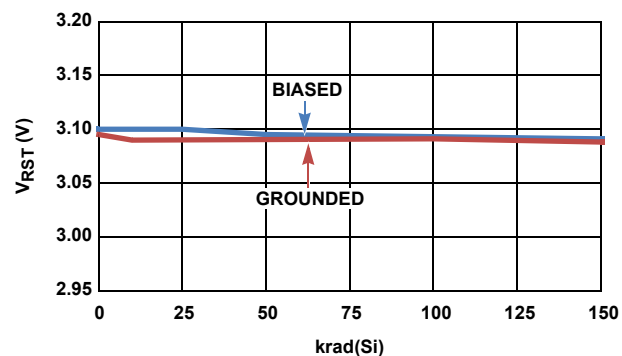
FIGURE 27. ISL706xEH V_{RST} vs LOW DOSE RATE RADIATION
