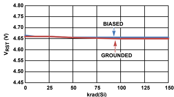
FIGURE 18. ISL705xEH V_{RST} vs LOW DOSE RATE RADIATION
