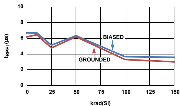
FIGURE 24. ISL705xEH t_{RPFI} vs LOW DOSE RATE RADIATION
