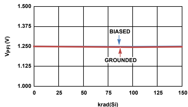
FIGURE 23. ISL705xEH V_{PFI} vs LOW DOSE RATE RADIATION
