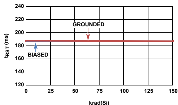
FIGURE 29. ISL706xEH t_{RST} vs LOW DOSE RATE RADIATION
