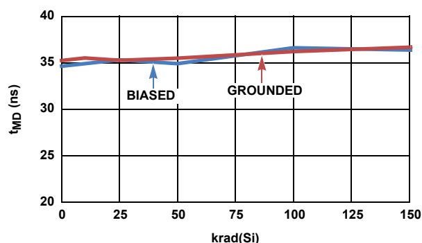
FIGURE 31. ISL706xEH t_{MD} vs LOW DOSE RATE RADIATION
