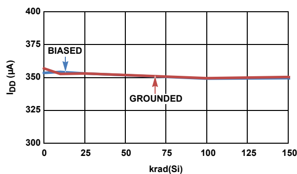
FIGURE 26. ISL706xEH I_{DD} vs LOW DOSE RATE RADIATION
