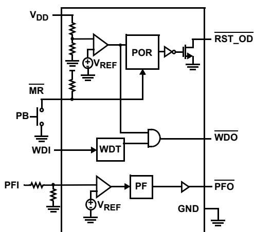
FIGURE 3C. ISL705CxH, ISL706CxH
