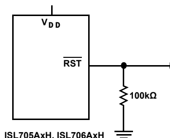
FIGURE 38. \overline{RST} VALID TO GROUND CIRCUIT
