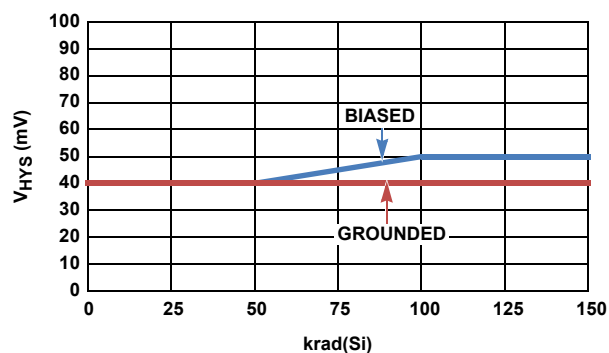
FIGURE 19. ISL705xEH V_{HYS} vs LOW DOSE RATE RADIATION
