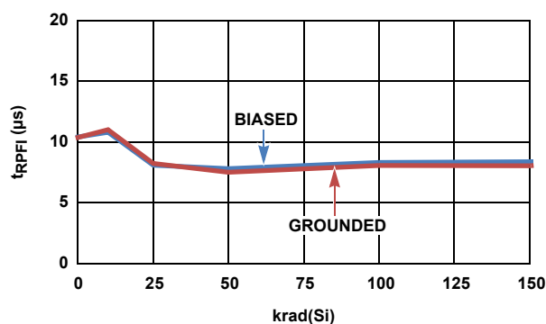
FIGURE 33. ISL706xEH t_{RPFI} vs LOW DOSE RATE RADIATION
