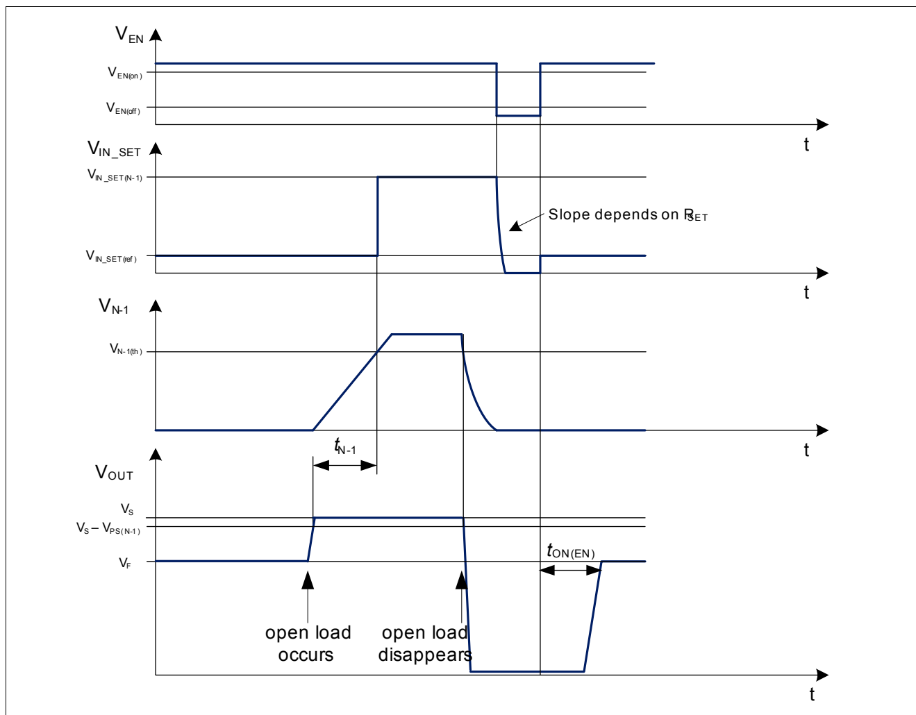
Figure 20 V_{IN\_SET} behavior during open load condition with ST pin connected to GND
