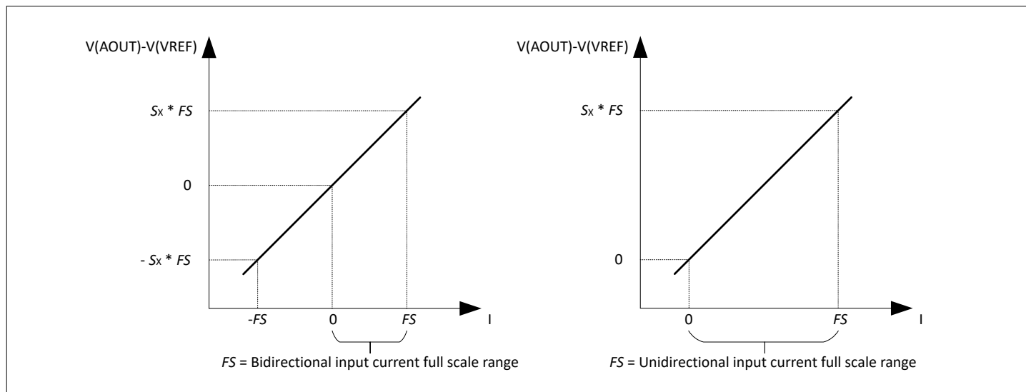
Figure 3 Full scale range definition (FS)
