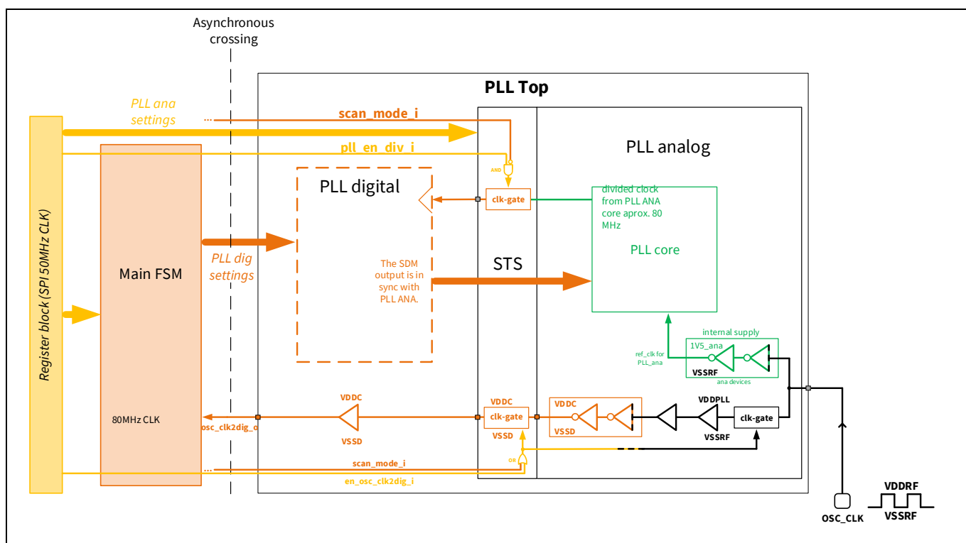
Figure 60 PLL and 80 MHz clock interface to the main FSM
