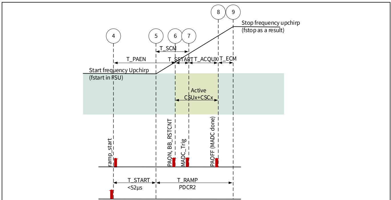
Figure 17 T_{\text{RAMP}} timing conditions
