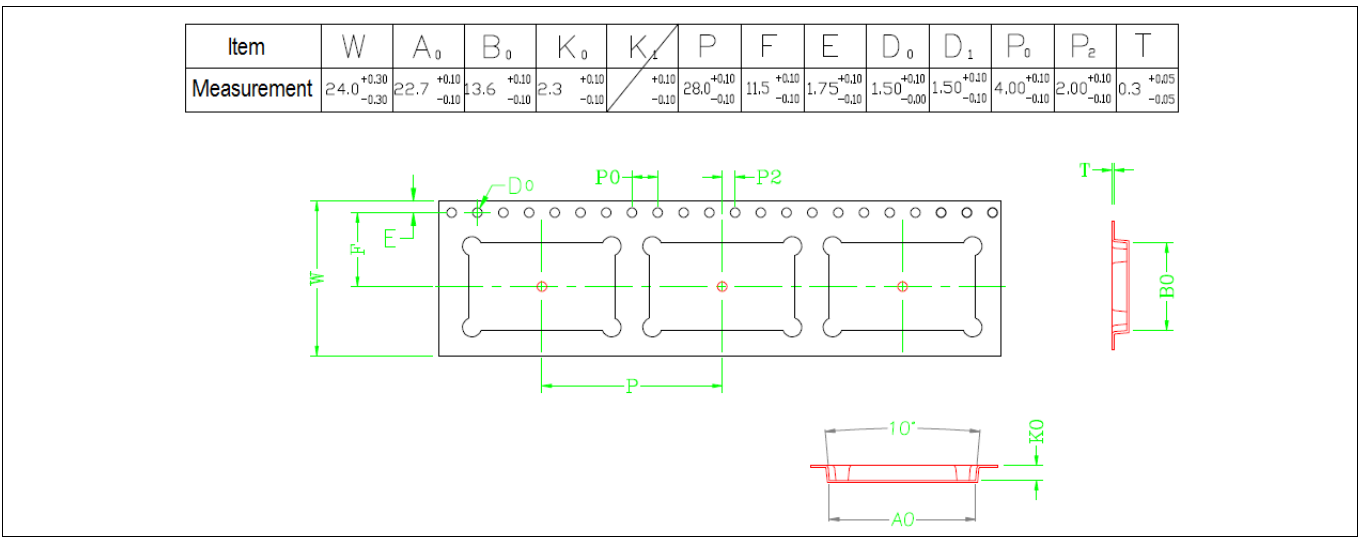
Figure 8 CYW20829B0-P4XXI100 tape dimensions
