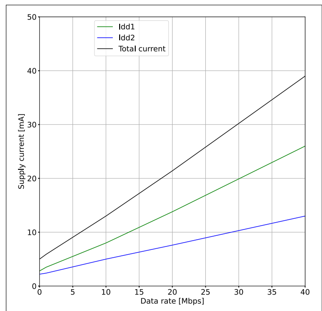
Figure 26 Supply current vs. data rate (V DD1 = V DD2 = 2.7 V)
