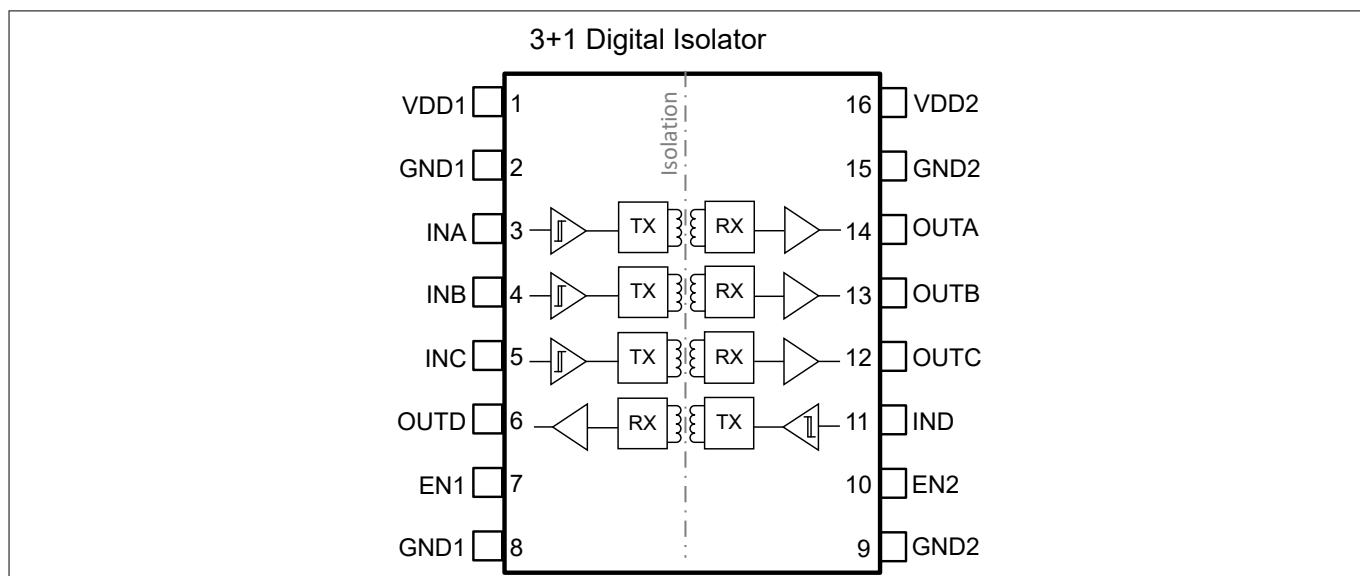
Figure 7 Pin-out for 4DIR140xHA
