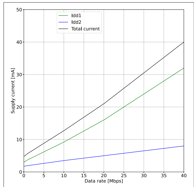
Figure 30 Supply current vs. data rate (V DD1 = V DD2 = 2.7 V)
