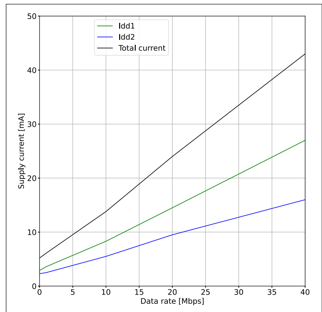
Figure 24 Supply current vs. data rate (V DD1 = V DD2 = 5 V)
