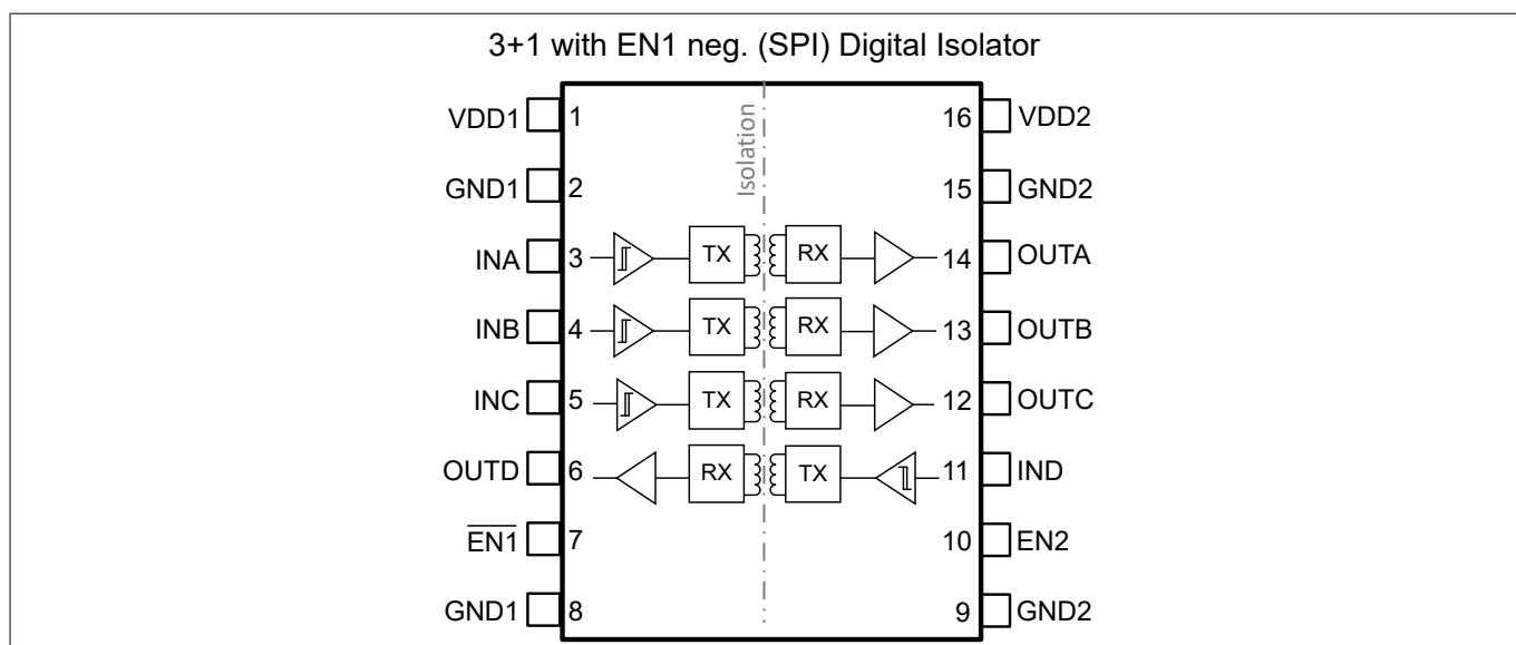
Figure 10 Pin-out for 4DIR142xHA
