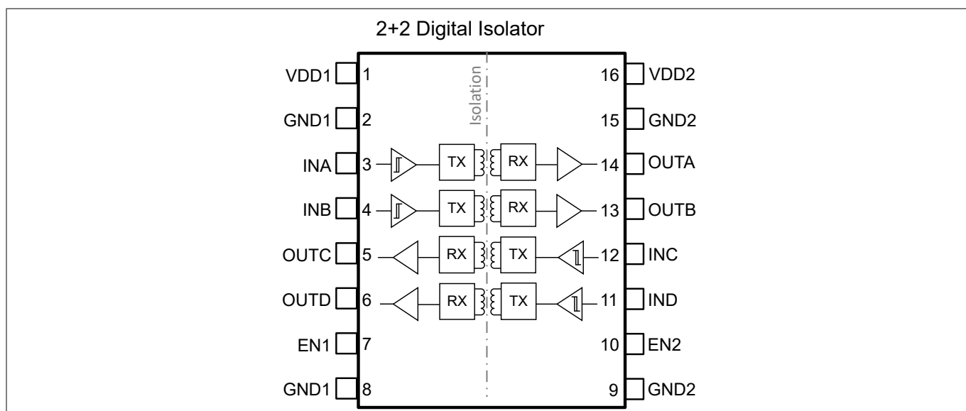
Figure 8 Pin-out for 4DIR240xHA
