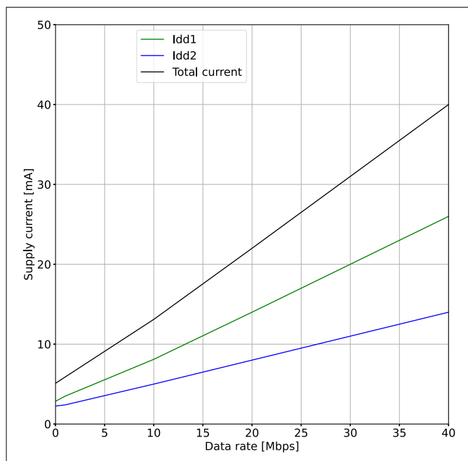
Figure 25 Supply current vs. data rate (V DD1 = V DD2 = 3.3 V)
