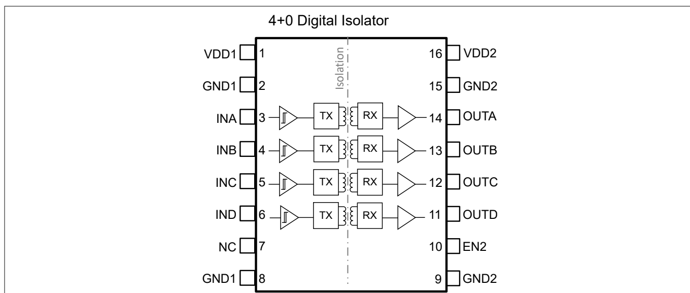
Figure 9 Pin-out for 4DIR040xHA
