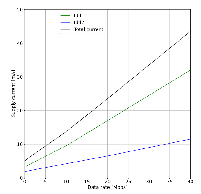
Figure 28 Supply current vs. data rate (V DD1 = V DD2 = 5 V)
