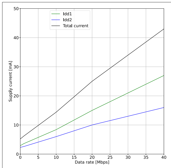
Figure 23 Supply current vs. data rate (V DD1 = V DD2 = 6.5 V)
