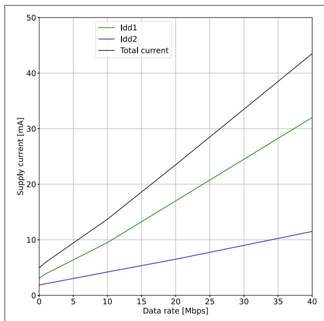
Figure 32 Supply current vs. data rate (V DD1 = V DD2 = 5 V)
