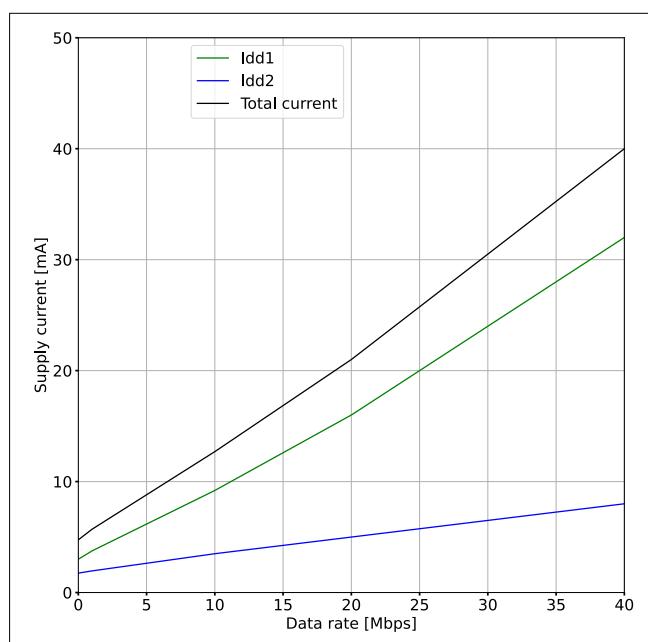
Figure 34 Supply current vs. data rate (V DD1 = V DD2 = 2.7 V)
