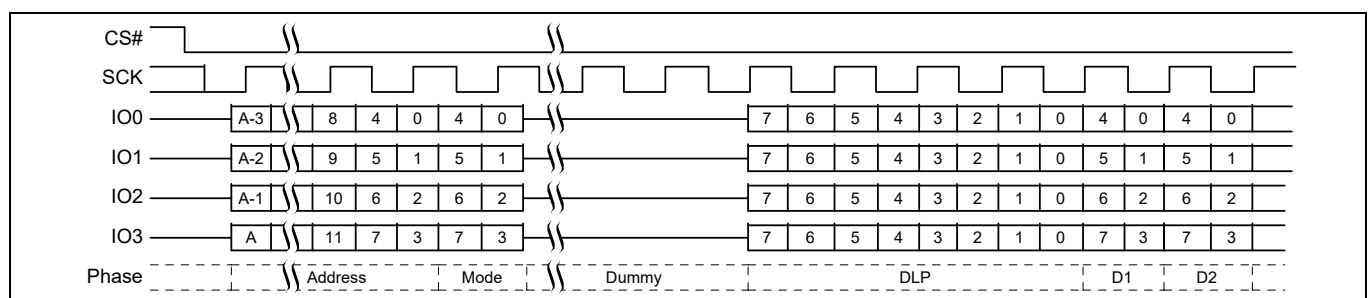
Figure 76 Continuous DDR Quad I/O Read subsequent access [40, 41, 42]
