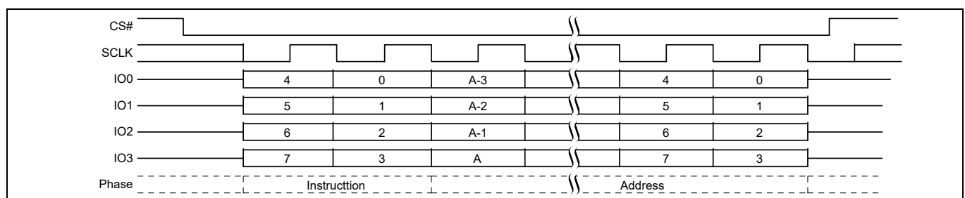
Figure 106 SPRP command sequence QPI mode [59, 60]
