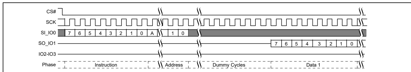
Figure 66 Fast Read (FAST_READ) command sequence [33]
