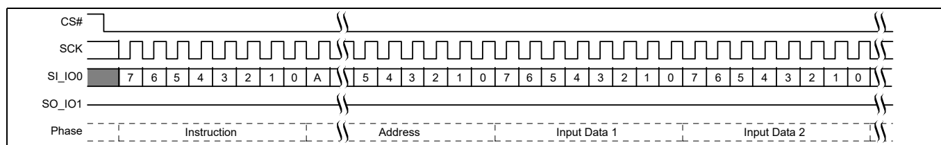
Figure 77 Page Program (PP 02h or 4PP 12h) command sequence [43]
