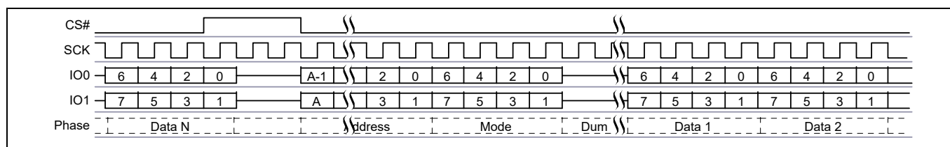
Figure 70 Dual I/O Continuous Read command sequence [36]
