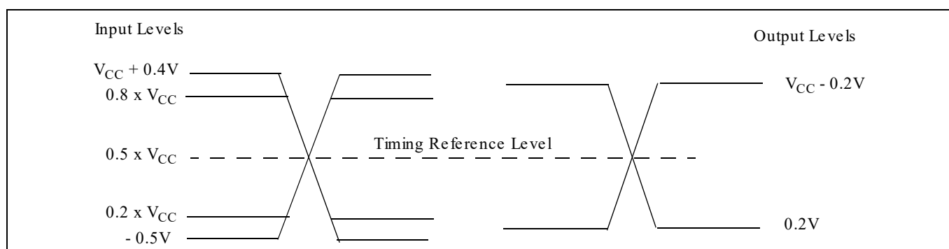
Figure 135 Input, output, and timing reference levels
