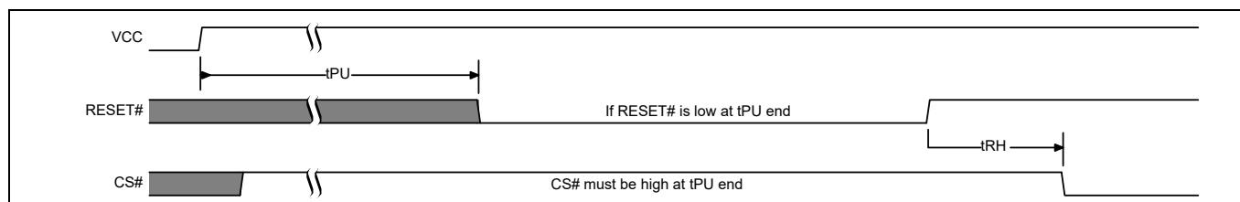
Figure 136 Reset low at the end of POR
