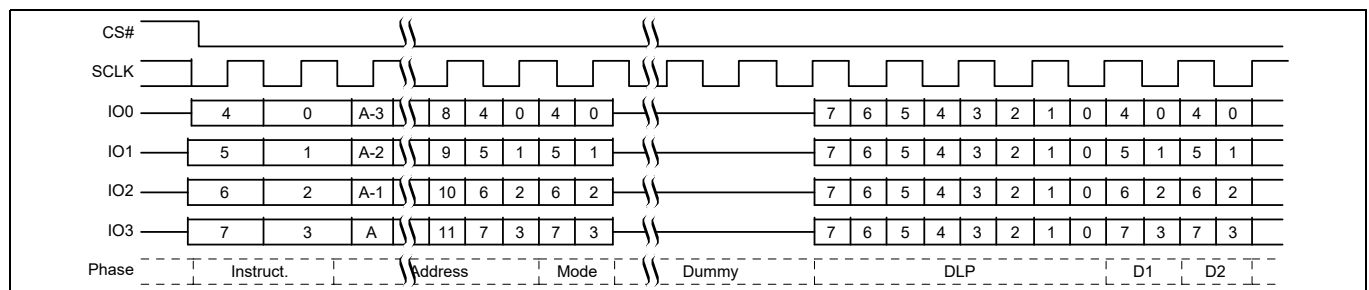
Figure 75 DDR Quad I/O Read initial access QPI mode [40, 42]
