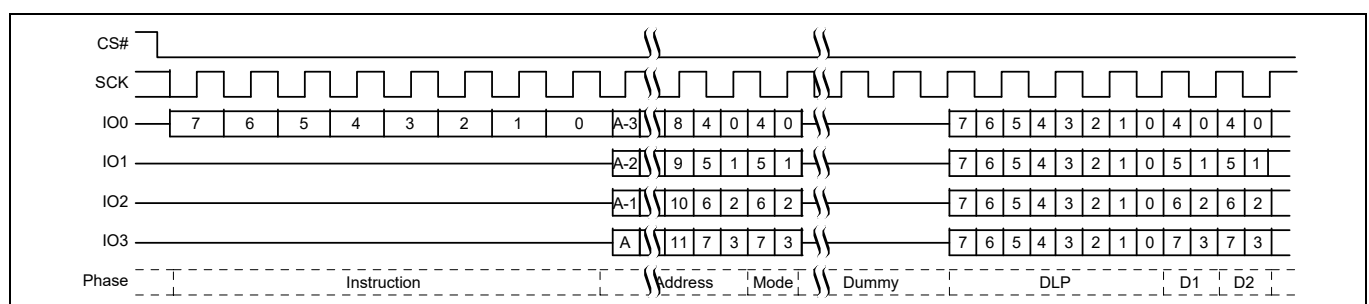
Figure 74 DDR Quad I/O Read initial access [40, 42]
