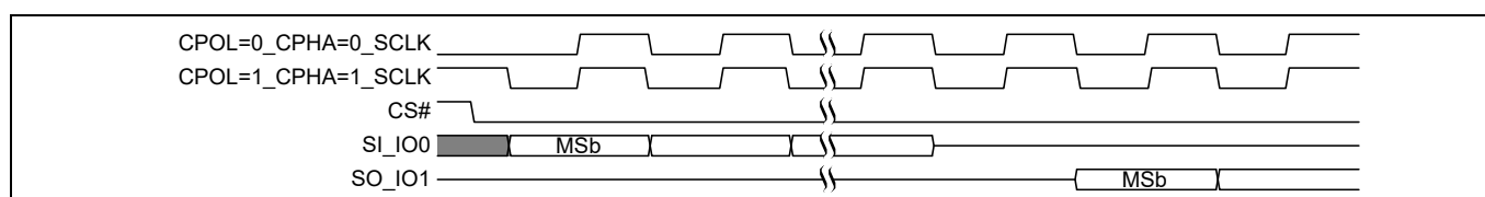
Figure 11 SPI SDR modes supported
