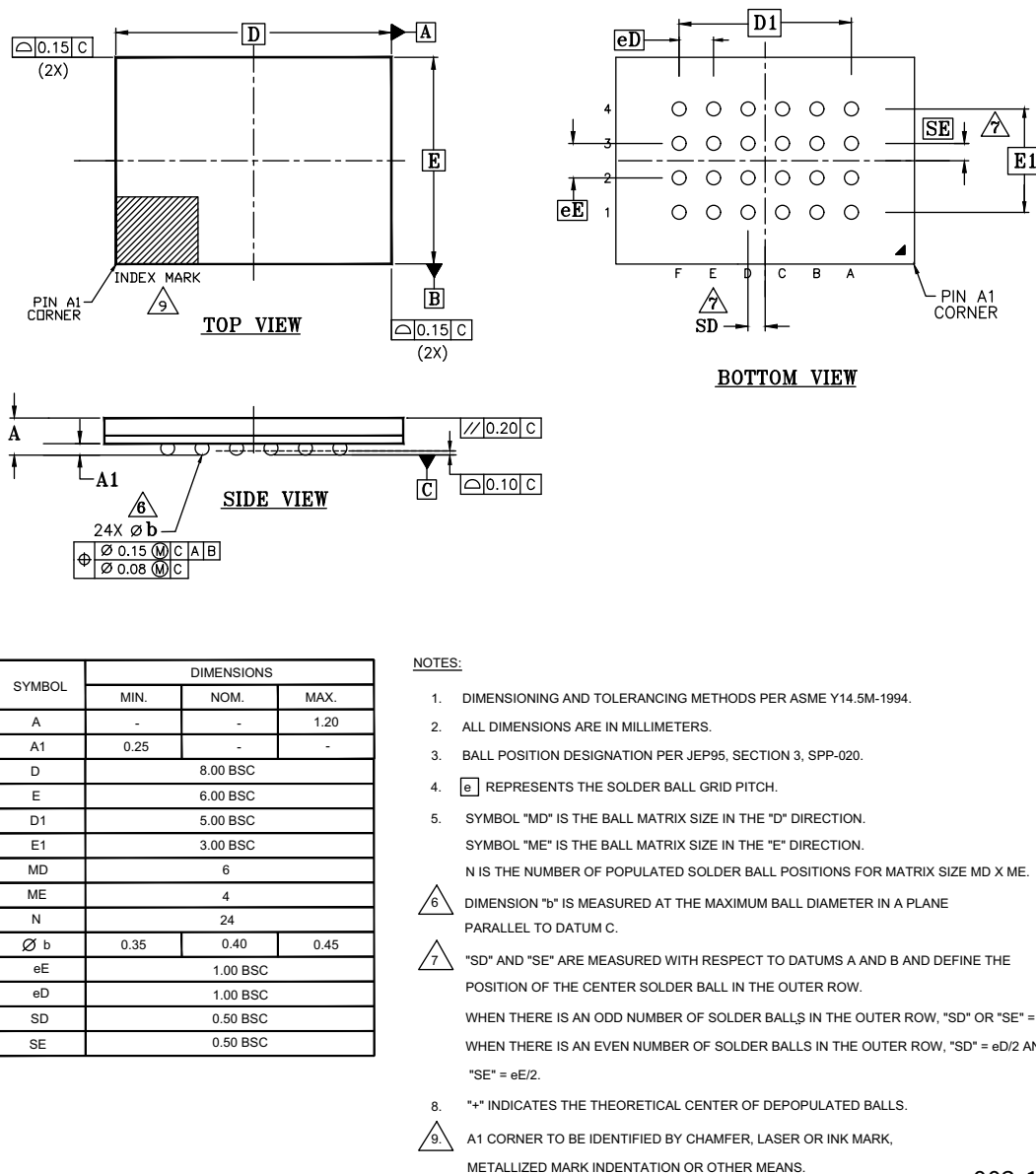
Figure 155 Ball grid array 24-ball 6 x 8 mm (FAC024)
