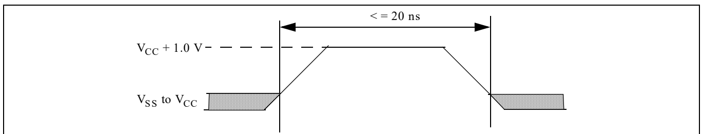
Figure 130 Maximum positive overshoot waveform
