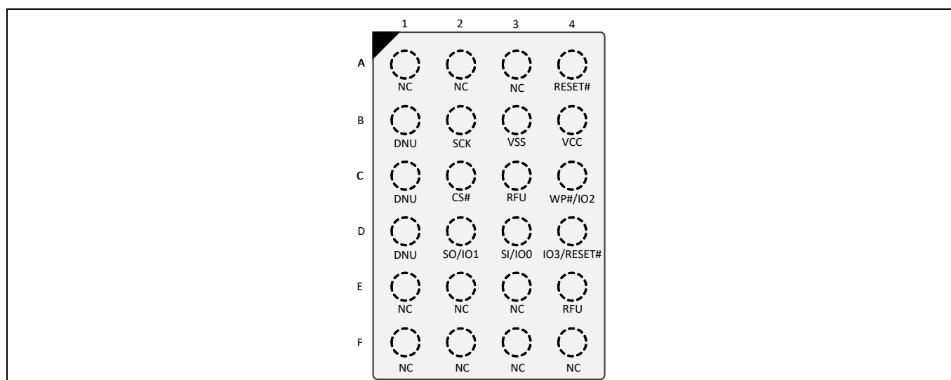
Figure 5 24-ball BGA, 4 x 6 ball footprint (FAC024), top view
