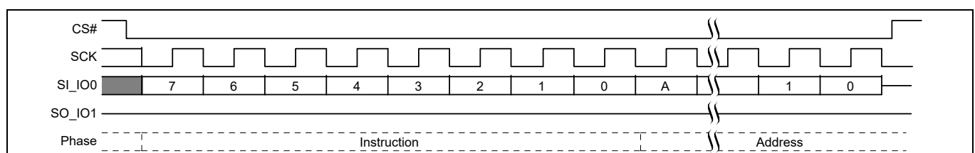
Figure 105 SPRP command sequence [59, 60]
