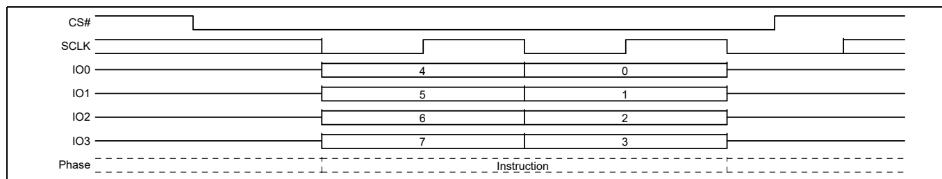
Figure 56 Enter 4 Byte Address QPI mode
