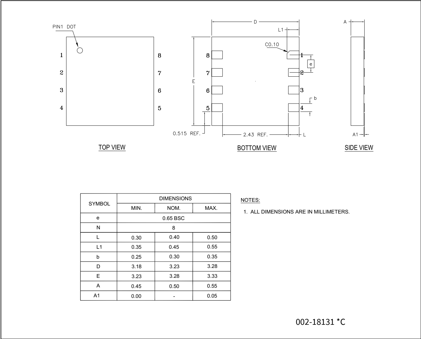
Figure 25 8-pin GQFN (3.23 × 3.28 × 0.55 mm) package outline, 002-18131
