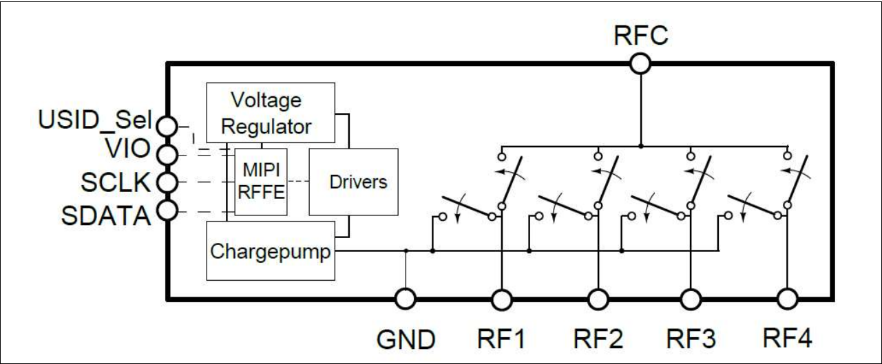
Figure 1 BGSA143ML10 Block diagram
