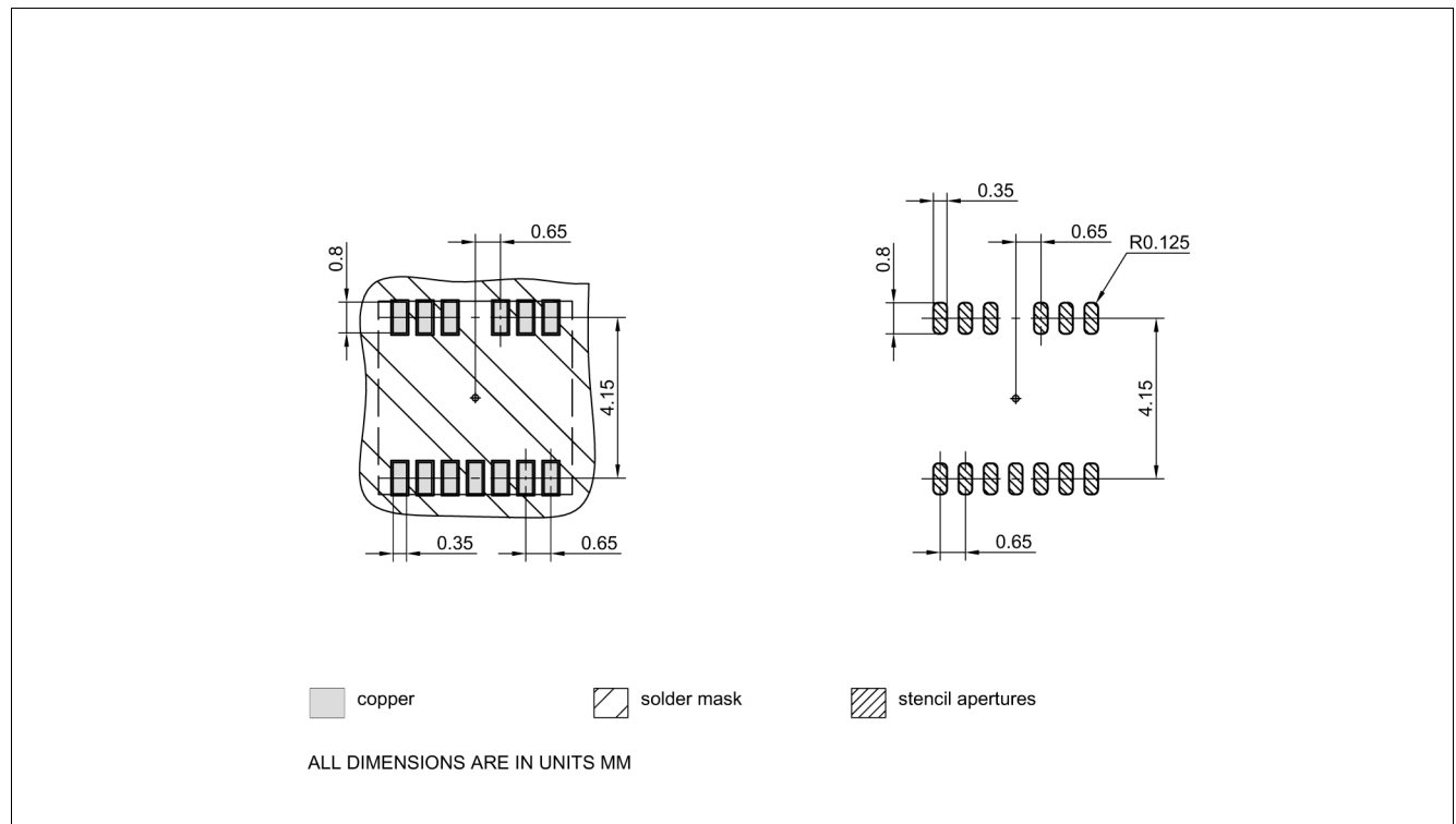
Figure 23 PG-TFLGA-13-1 footprint
