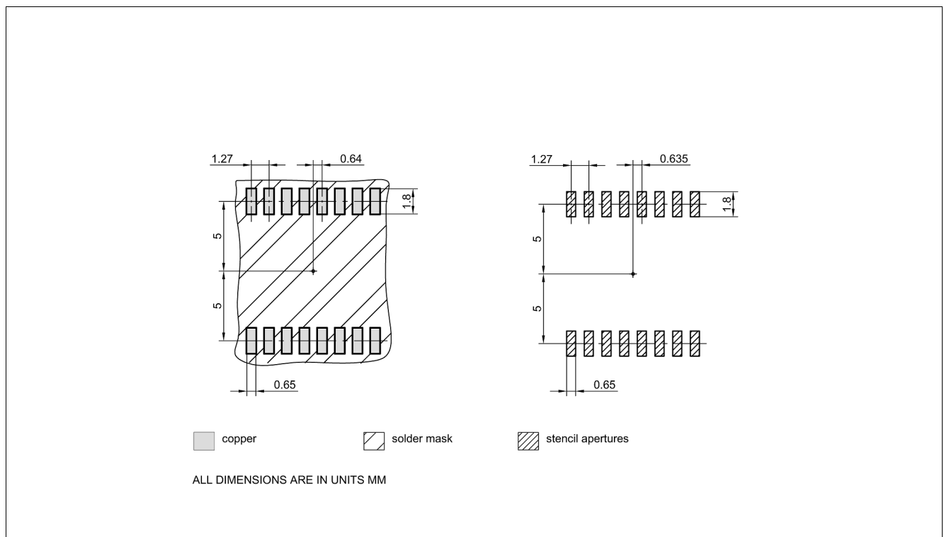
Figure 20 PG-DSO-16-30 footprint
