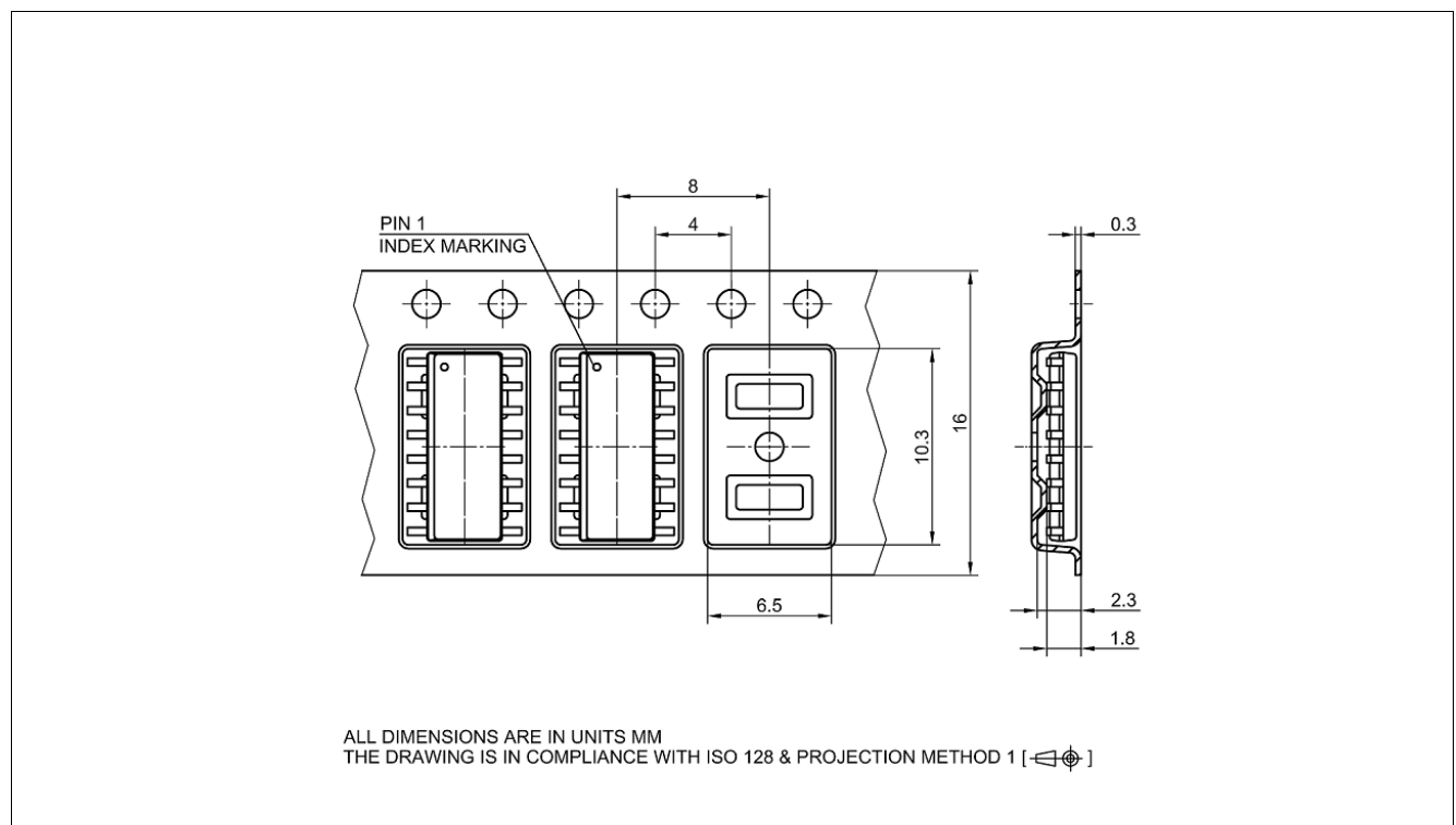
Figure 18 PG-DSO-16-11 packaging
