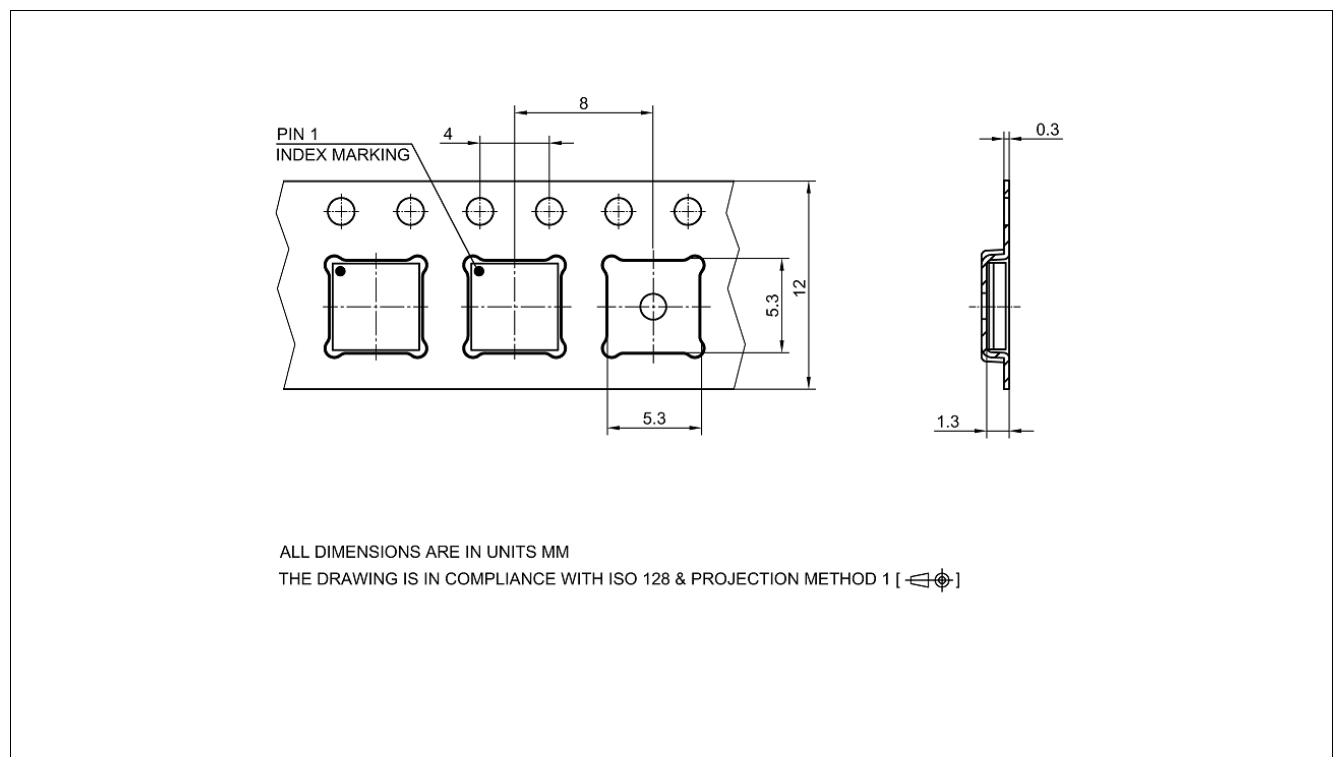
Figure 24 PG-TFLGA-13-1 packaging
