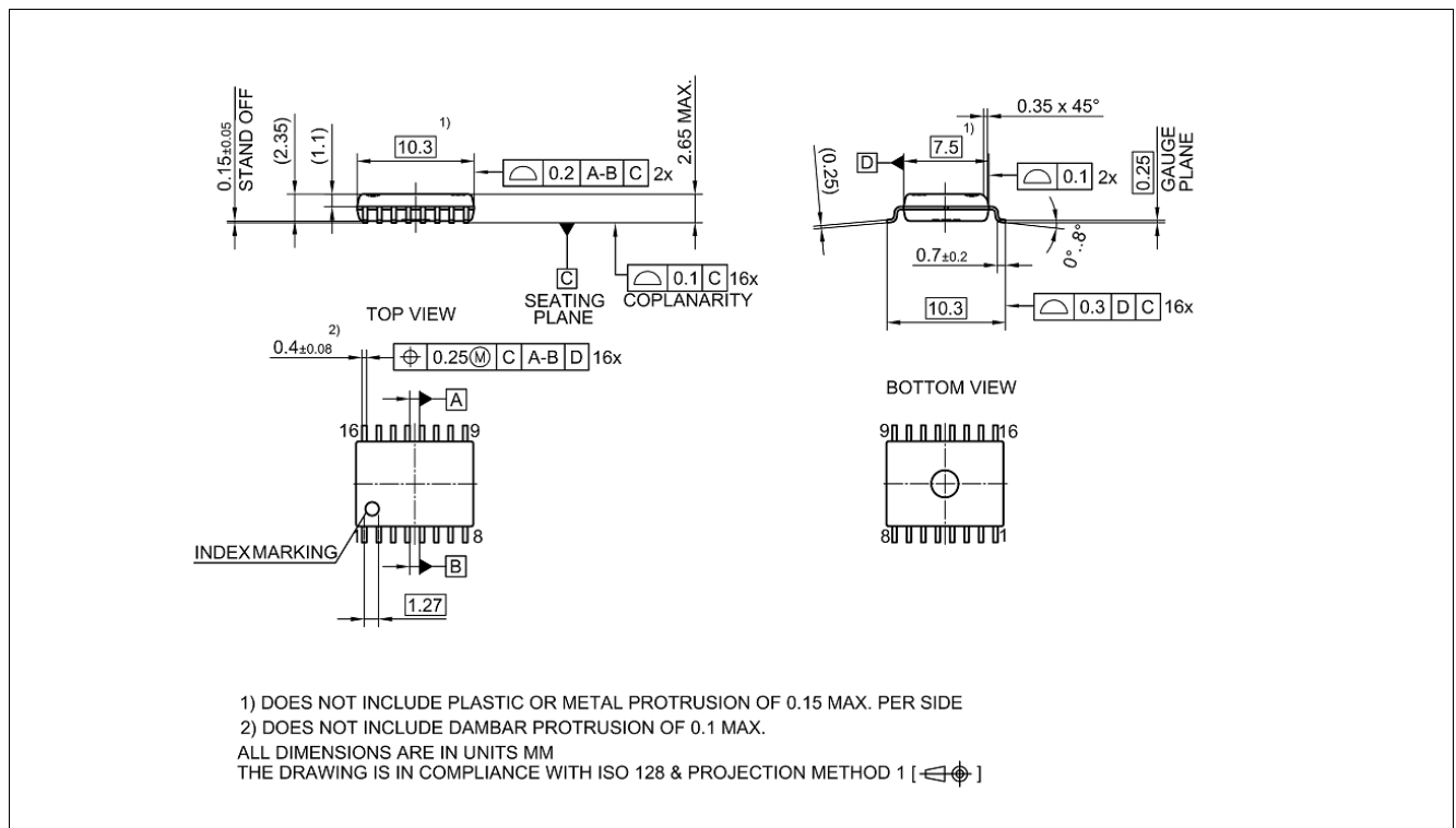
Figure 19 PG-DSO-16-30 outline
