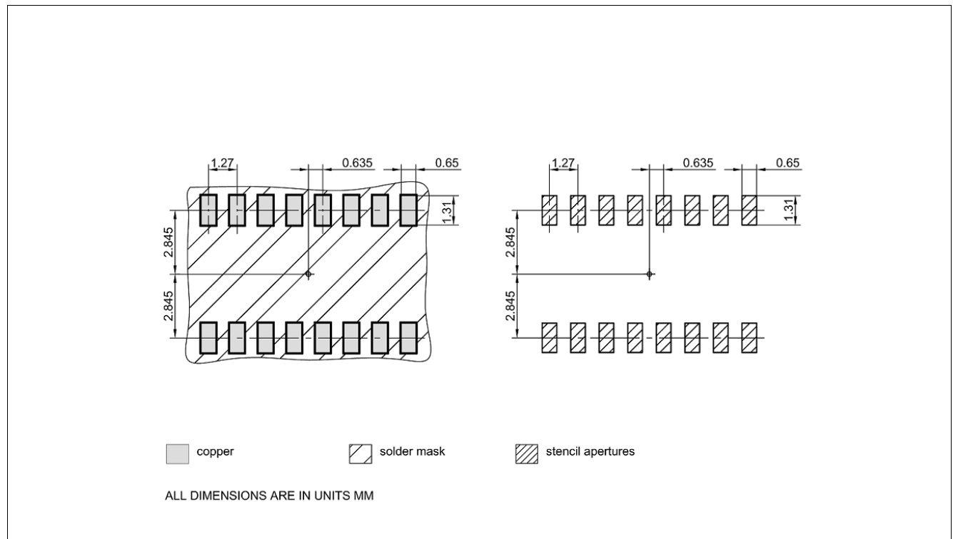
Figure 17 PG-DSO-16-11 footprint
