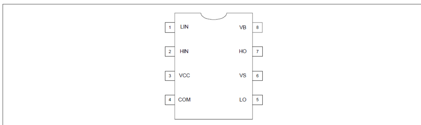
Figure 3 2ED2304S06F lead assignments (DSO-8)
