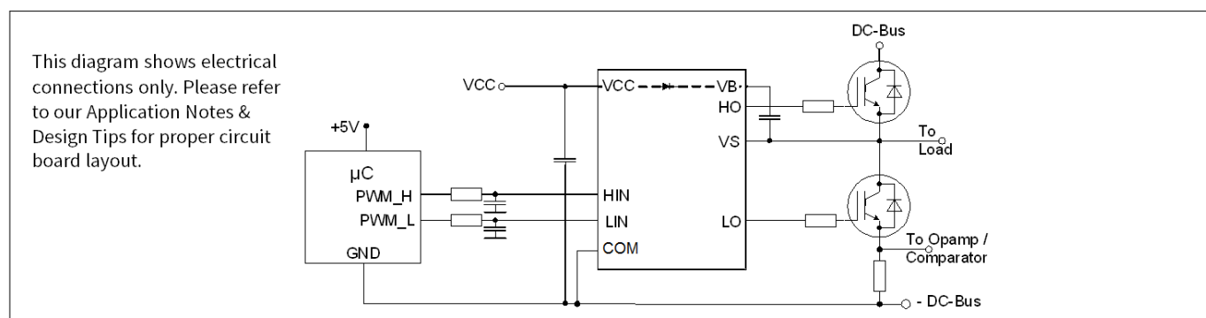
Figure 1 Typical connection diagram
