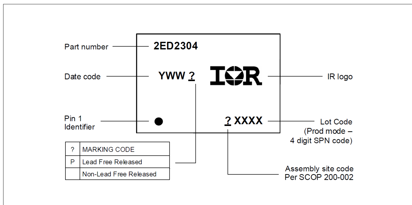
Figure 5 Marking information PG-DSO-8 (2ED2304S06F)
