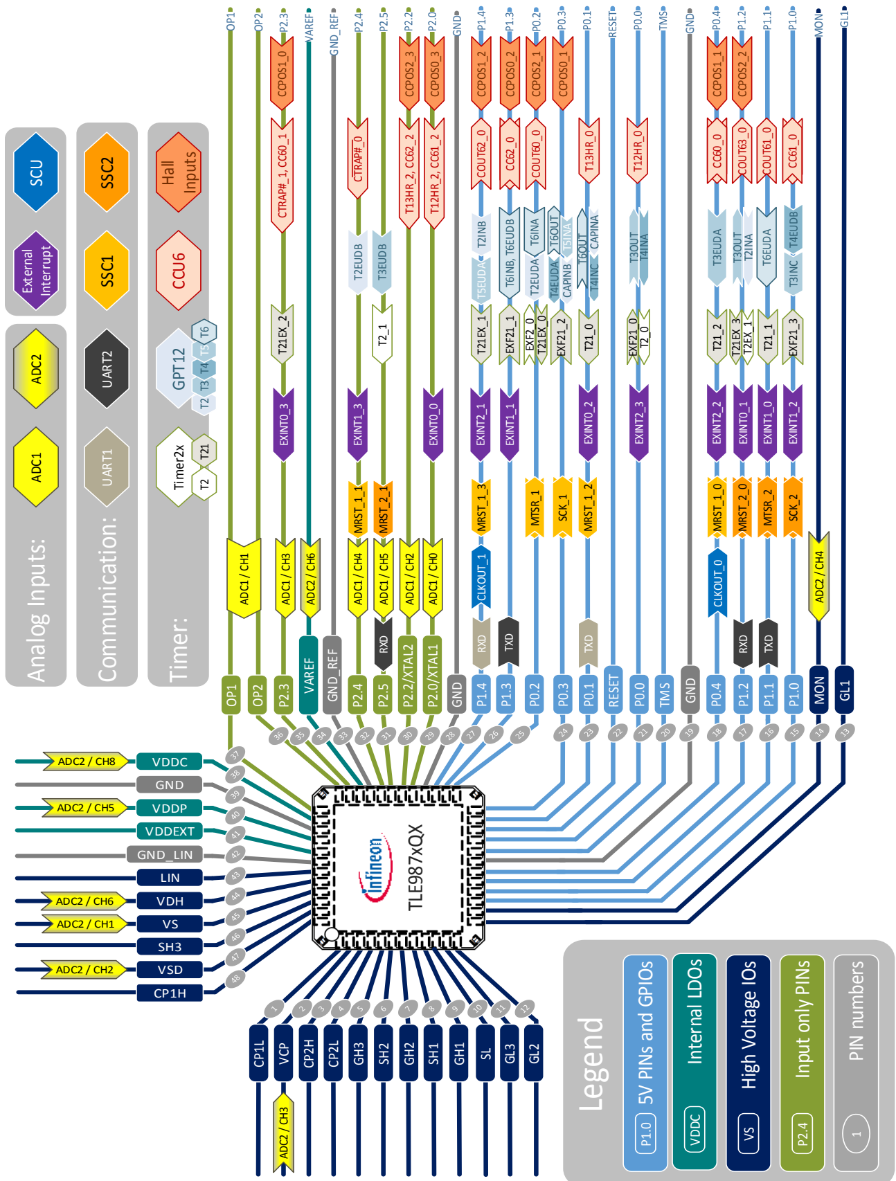
Figure 81 Alternate Function Map
