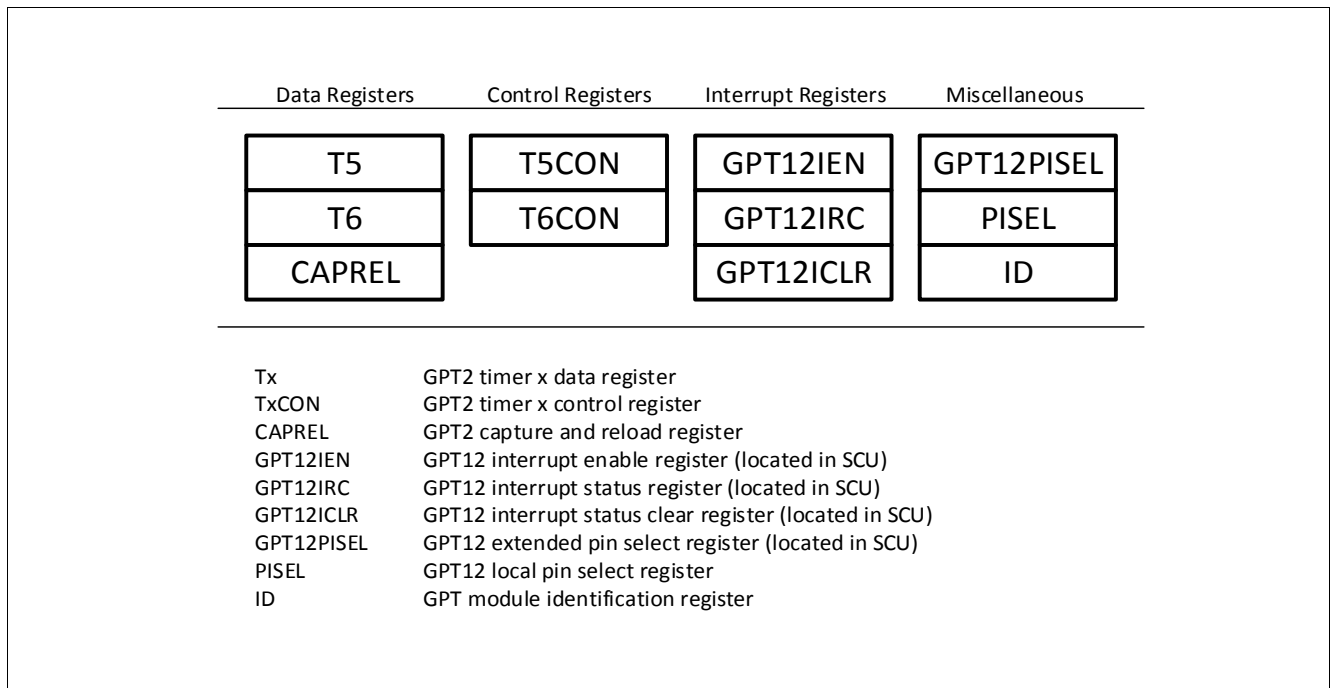
Figure 101 SFRs Associated with Timer Block GPT2
