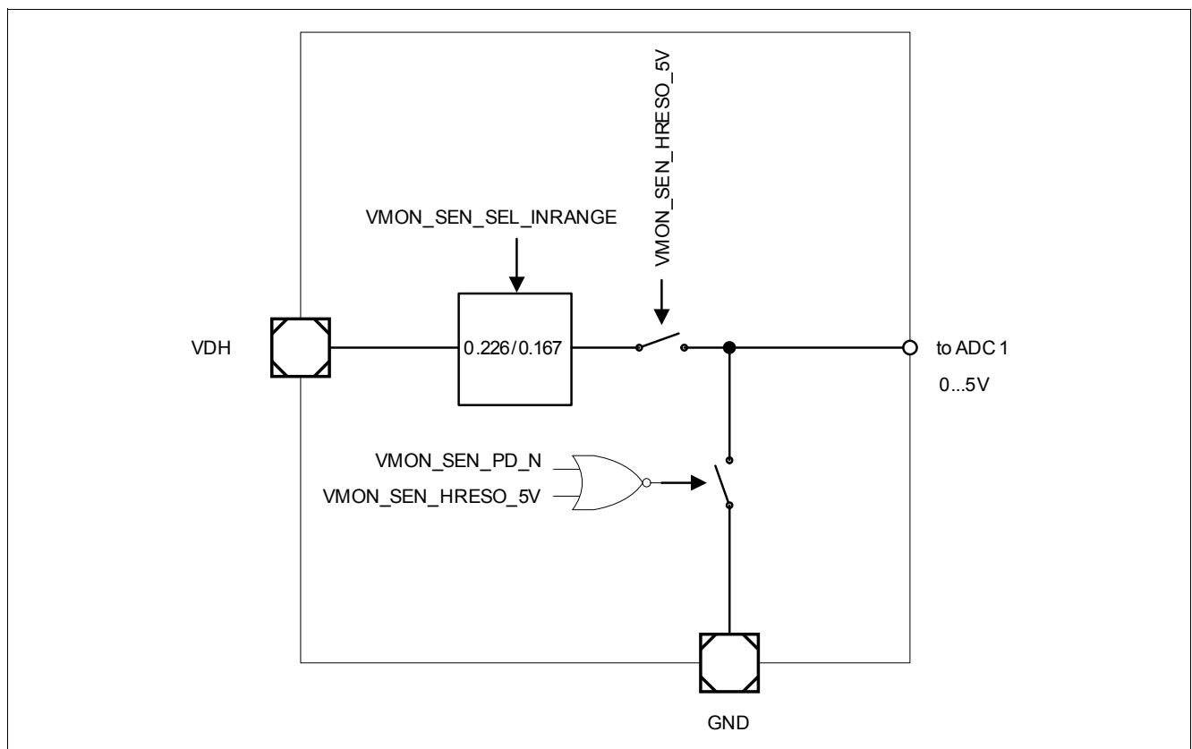
Figure 193 Input Structure of HV-VDH Attenuator
