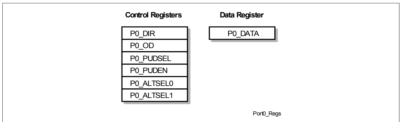
Figure 78 Port 0 Registers
