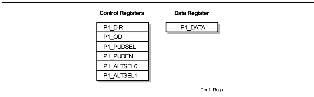
Figure 79 Port 1 Registers
