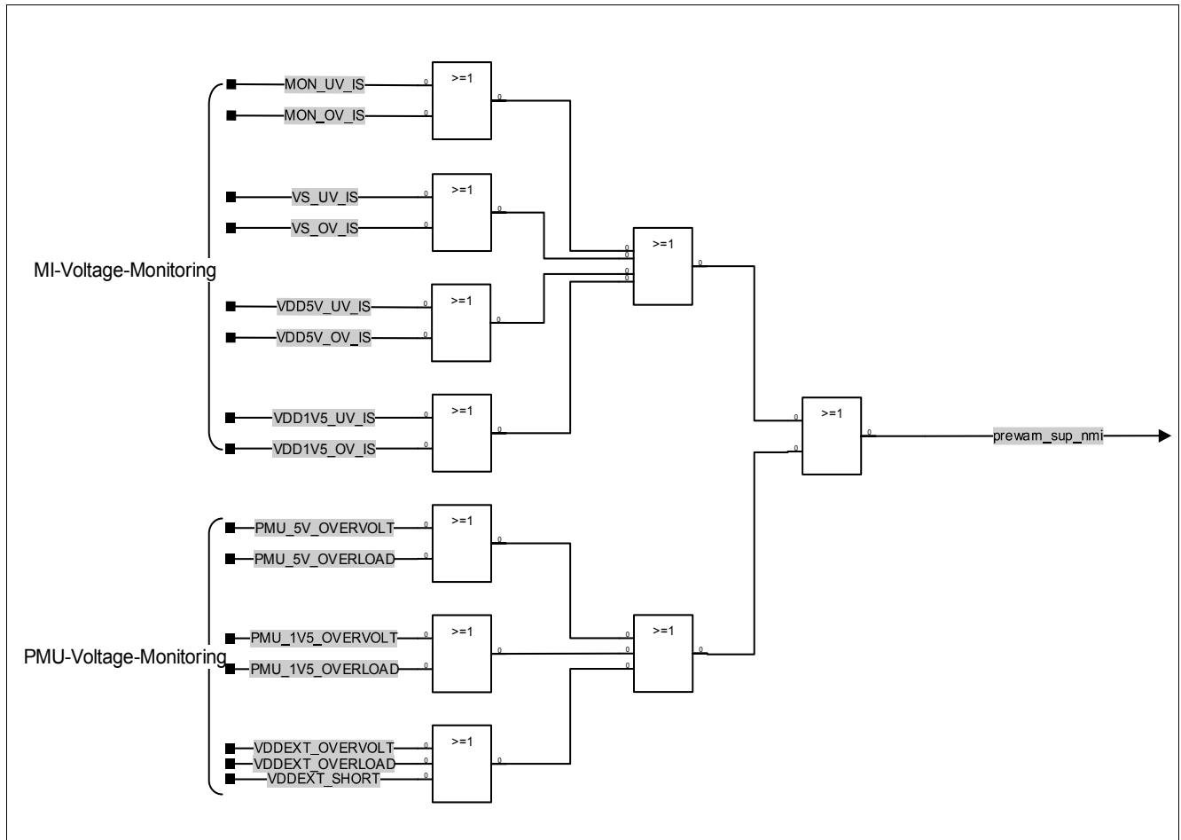
Figure 38 Structure of PREWARN_SUP
