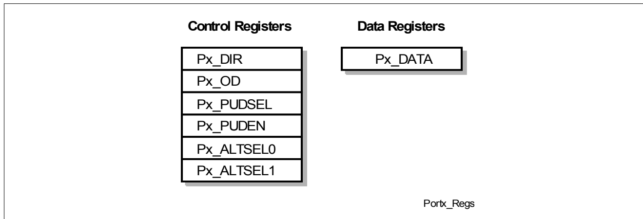
Figure 77 Port Registers
