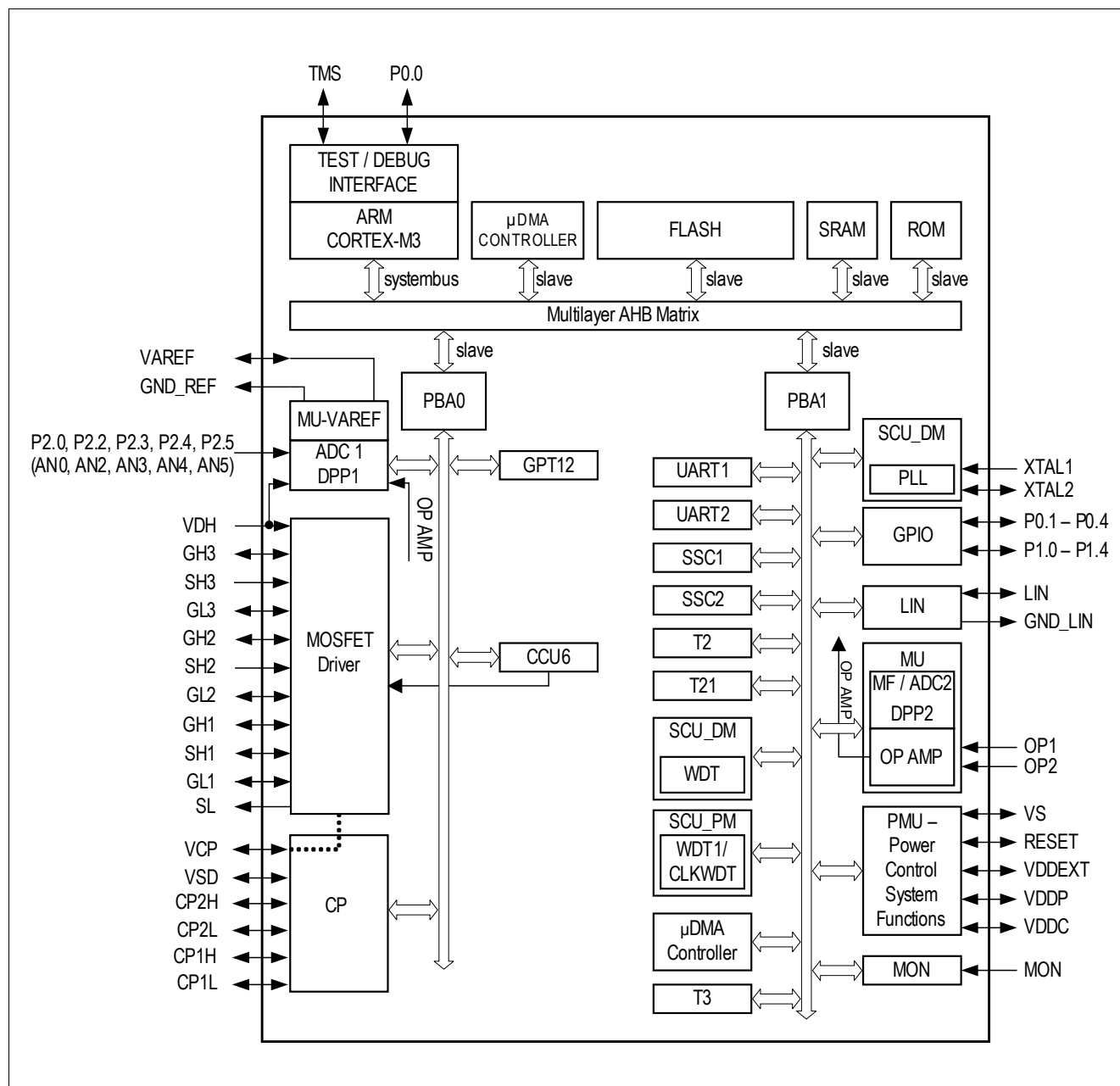
Figure 1 Block Diagram TLE987xQX, except TLE9871 variants
