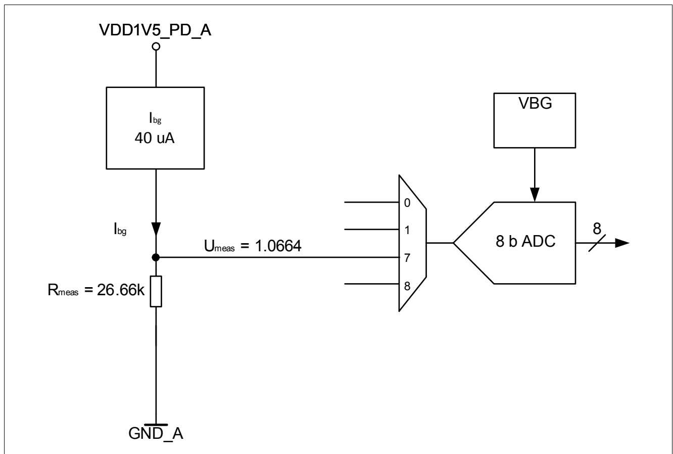
Figure 198 Principle of ADC2 functional safety feature
