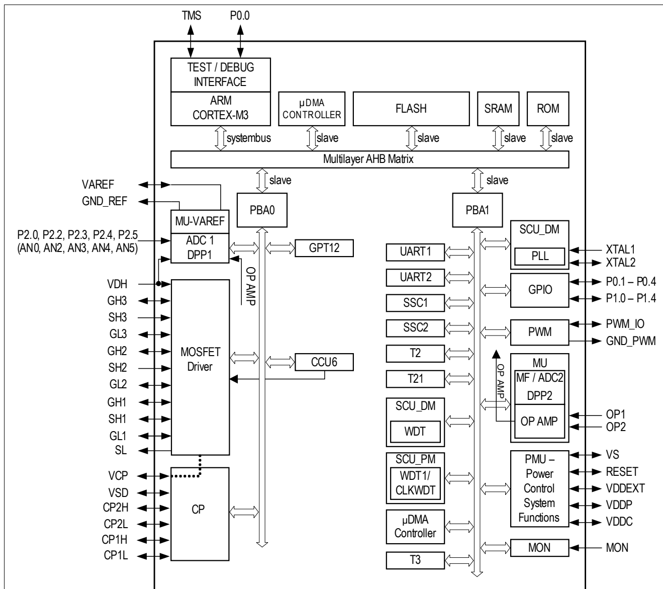
Figure 2 Block Diagram TLE9871 variants only
