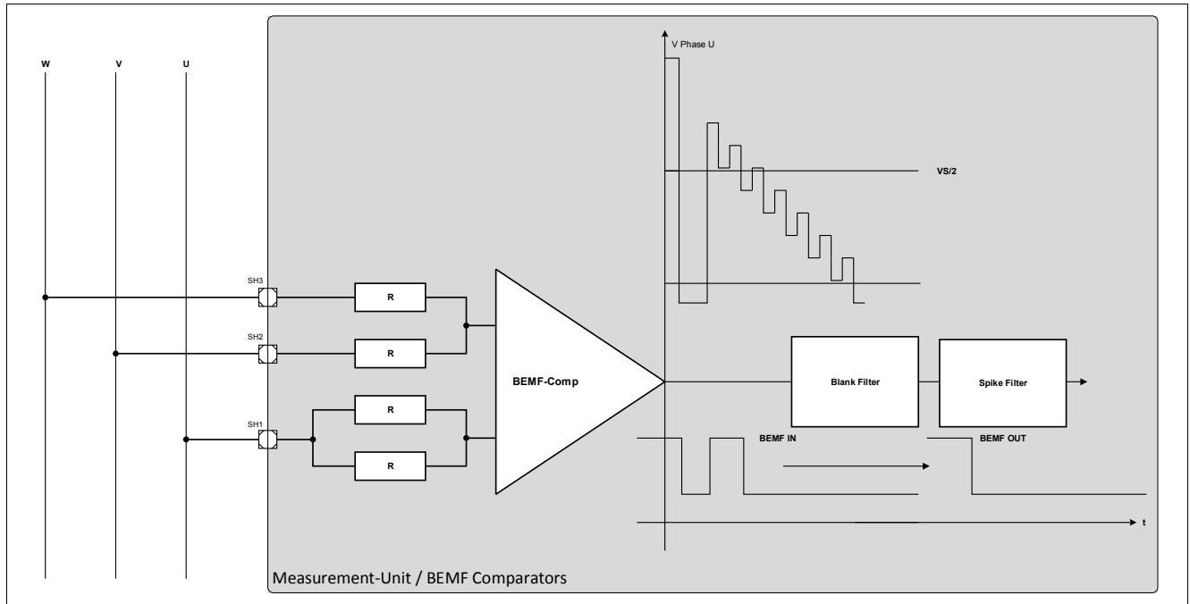
Figure 191 3 Times BEMF Comparator
