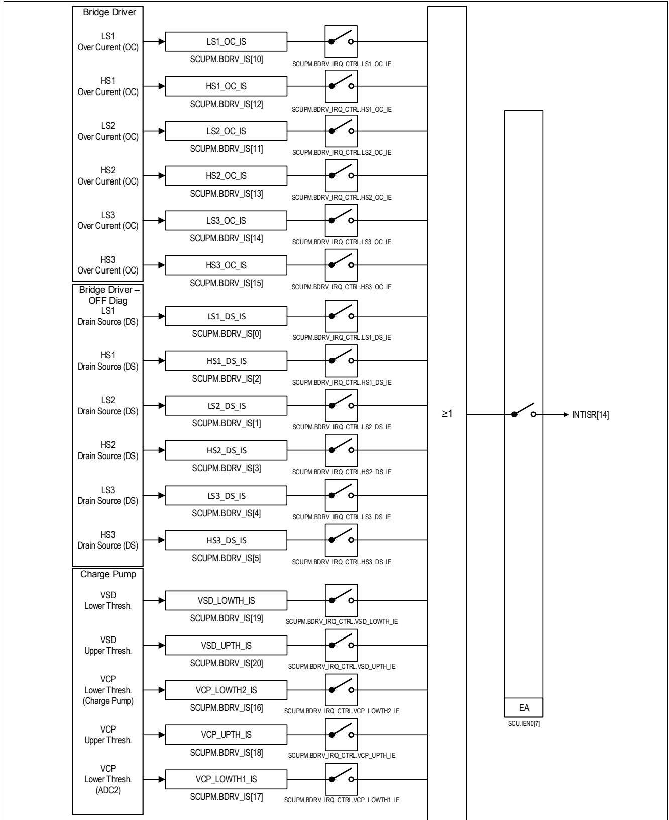
Figure 66 Interrupt Request Sources 14 (Bridge Driver)
