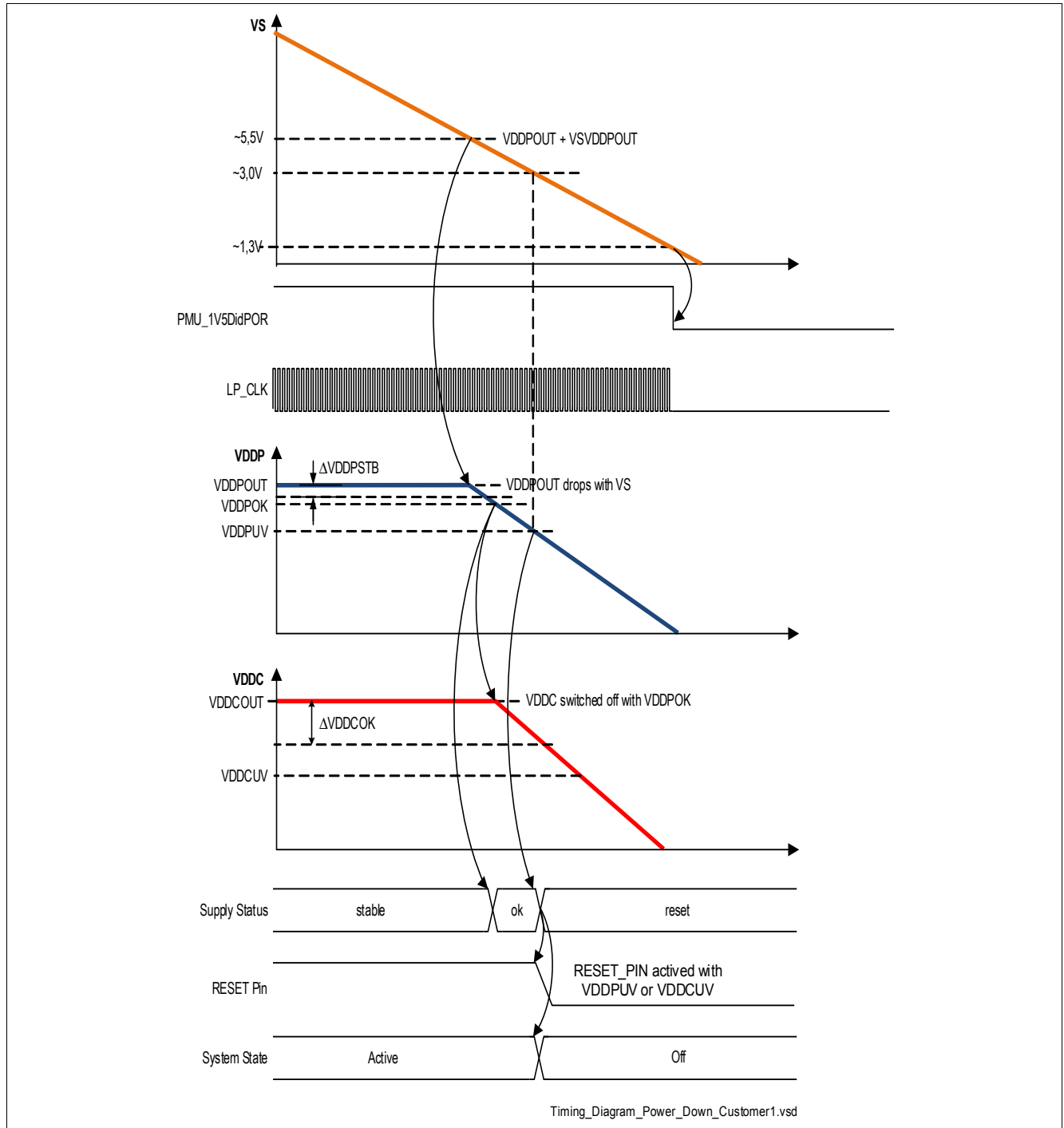
Figure 21 Power-Down and Power Loss Sequence
