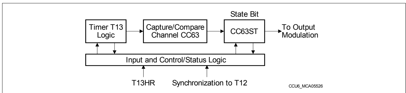
Figure 147 Overview Diagram of the Timer T13 Block
