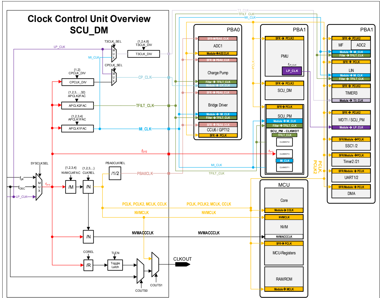
Figure 28 Clock Tree
