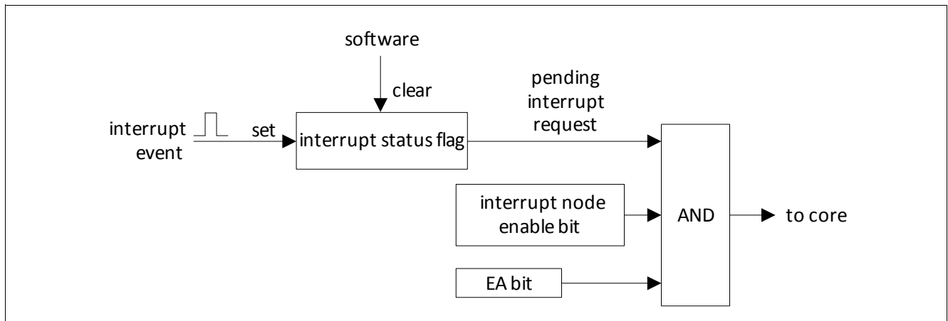
Figure 69 Interrupt Structure 1
