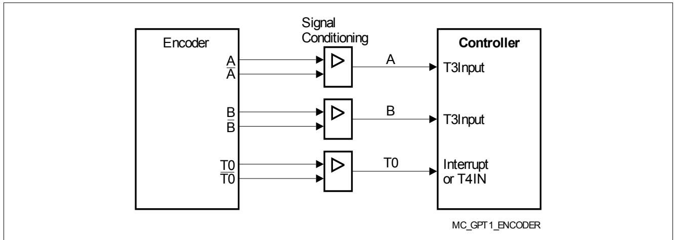
Figure 90 Connection of the Encoder to the TLE987xQX
