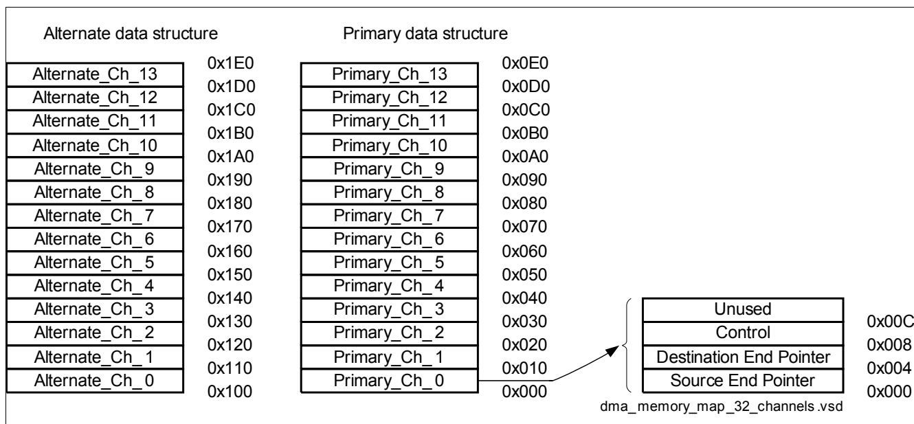
Figure 49 Memory Map for 32 Channels, Including the Alternate Data Structure
