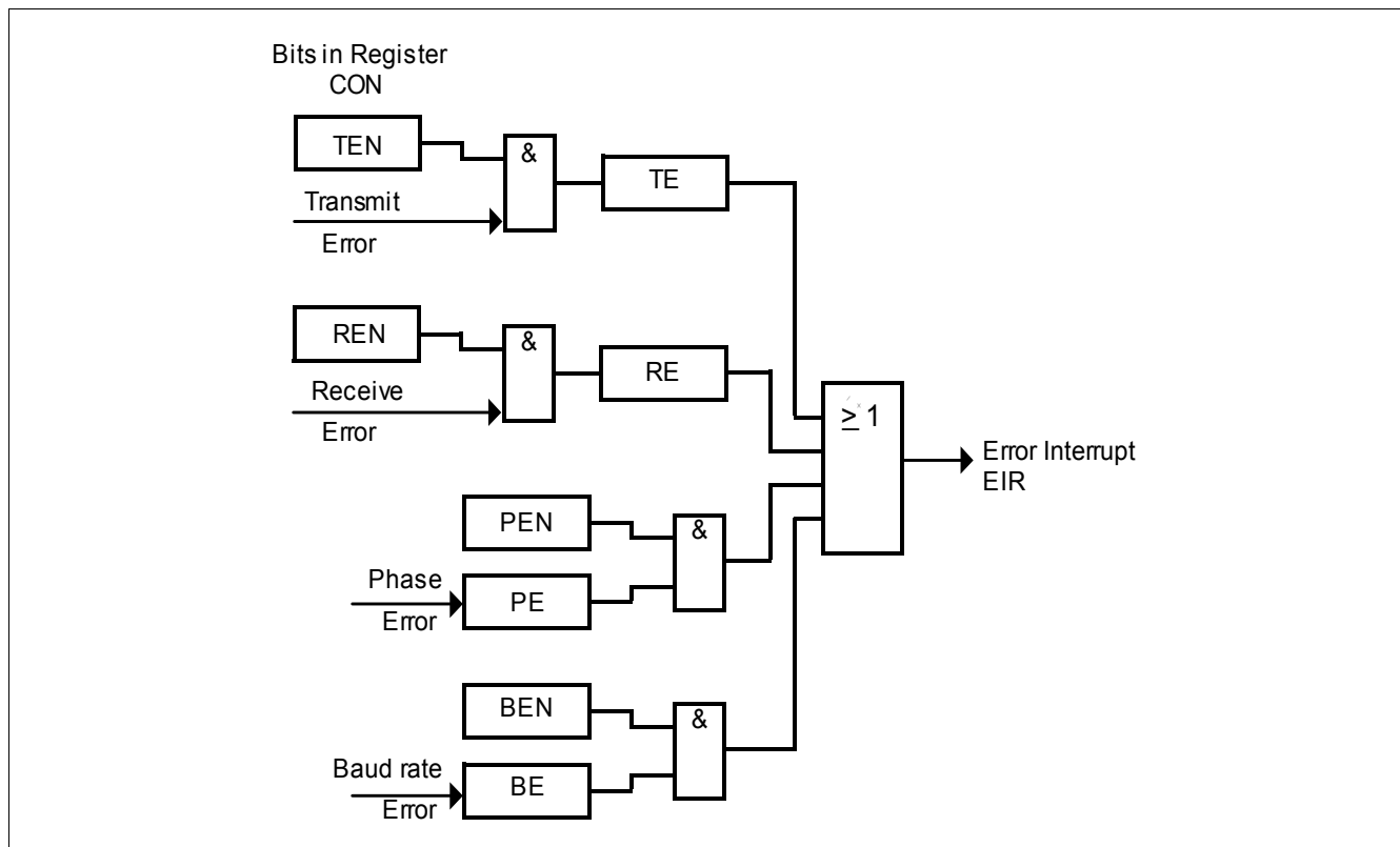
Figure 187 SSC Error Interrupt Control
