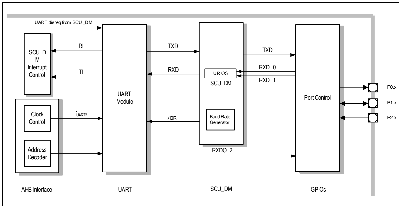
Figure 168 UART Block Diagram
