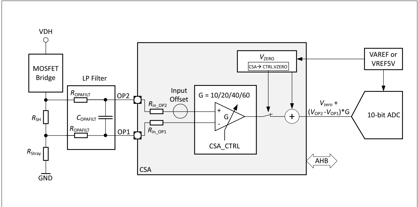
Figure 227 Simplified Application Diagram
