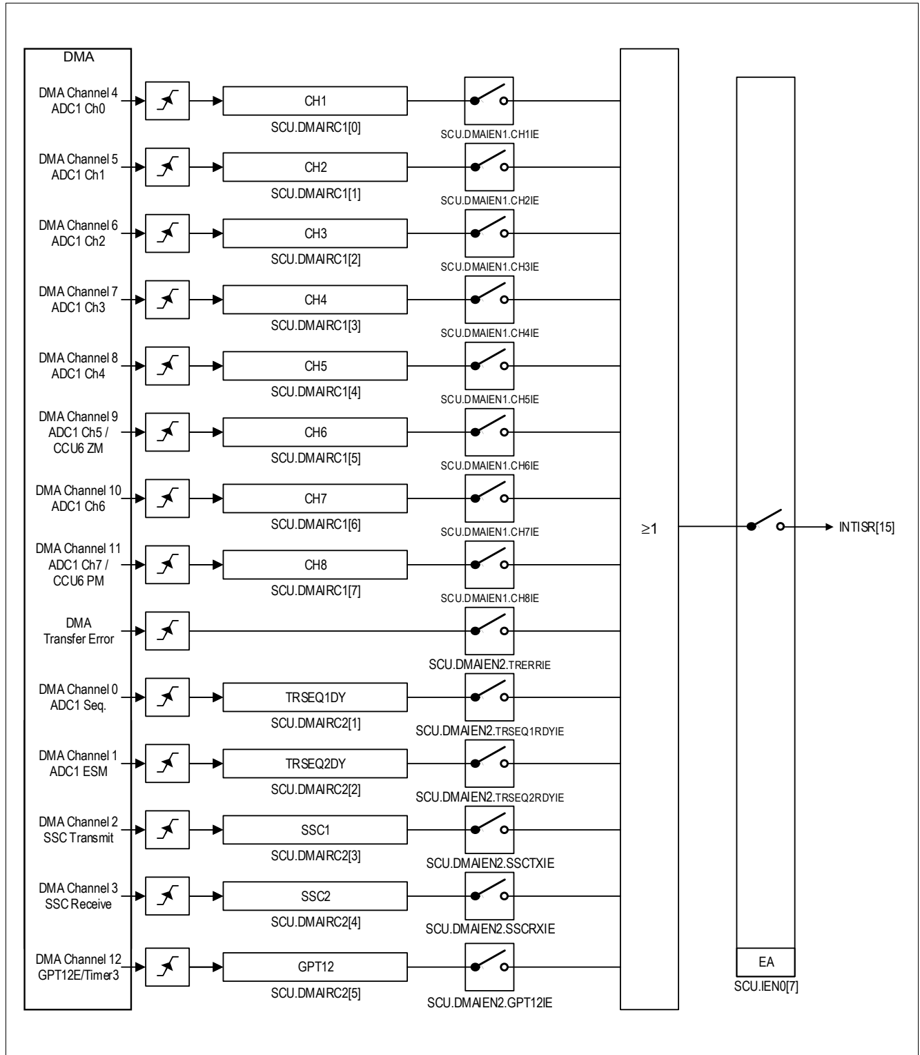
Figure 67 Interrupt Request Sources 15 (DMA)
