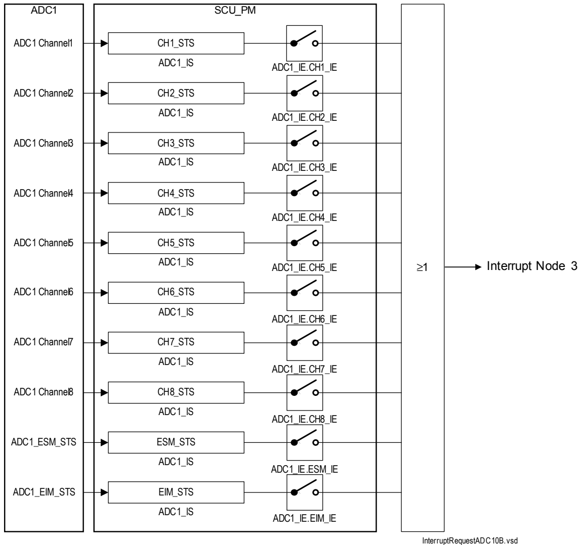
Figure 207 ADC1 Interrupt Generation
