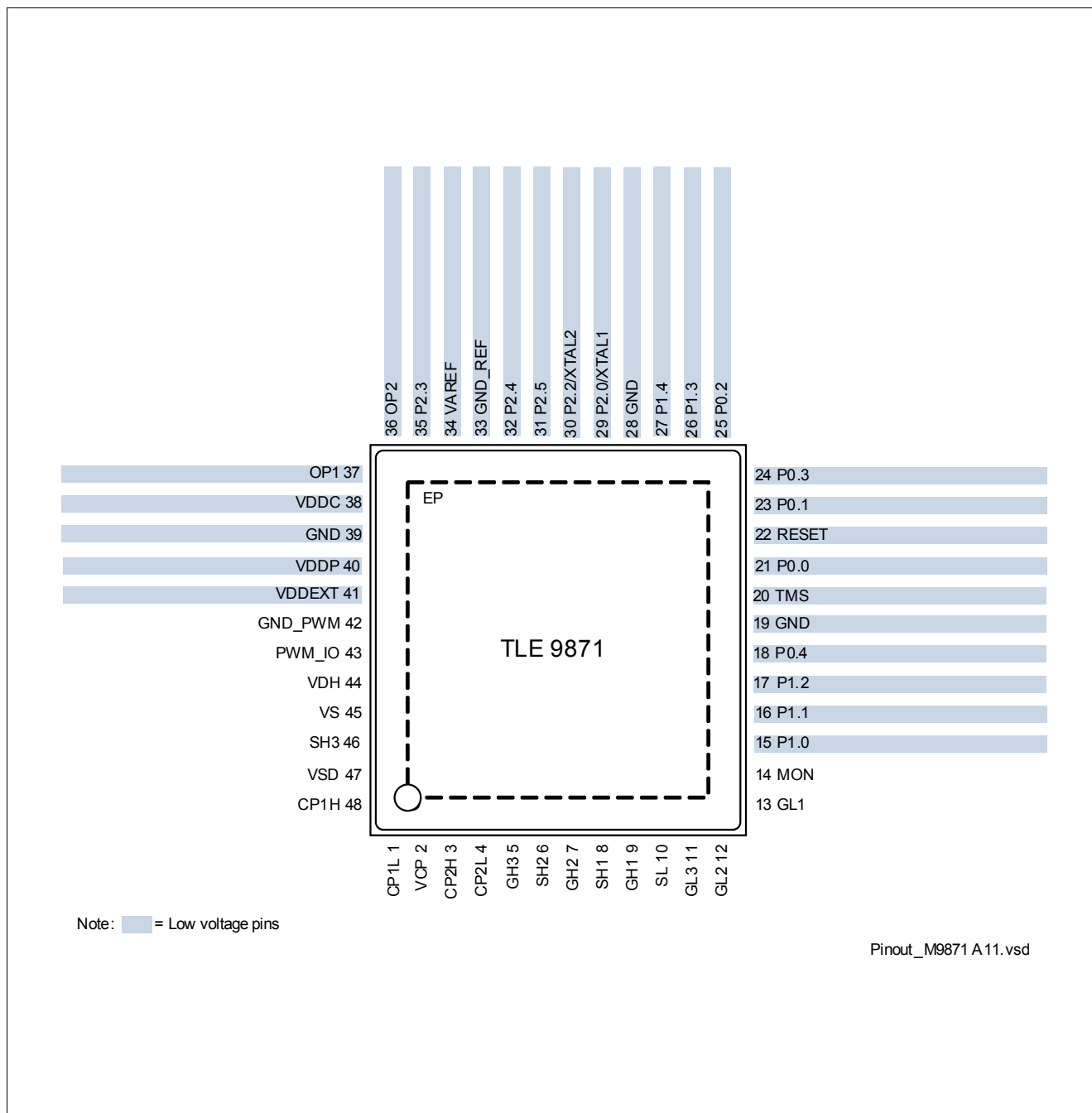
Figure 4 Device Pinout, TLE9871 variants only
