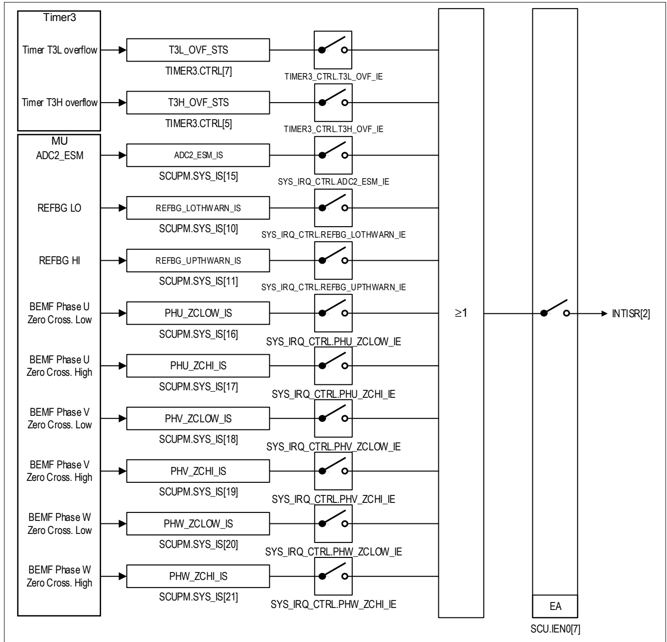
Figure 58 Interrupt Request Sources 2 (MU)
