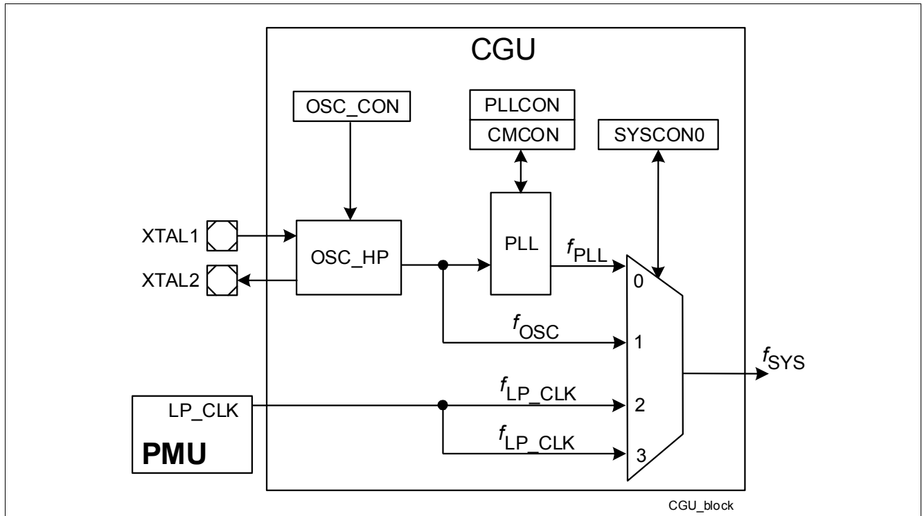
Figure 24 Clock Generation Unit Block Diagram
