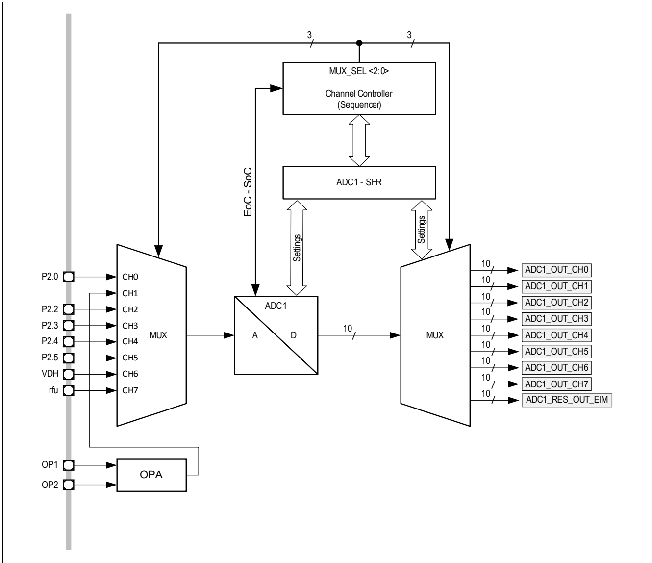
Figure 206 ADC1 Top Level Block Diagram
