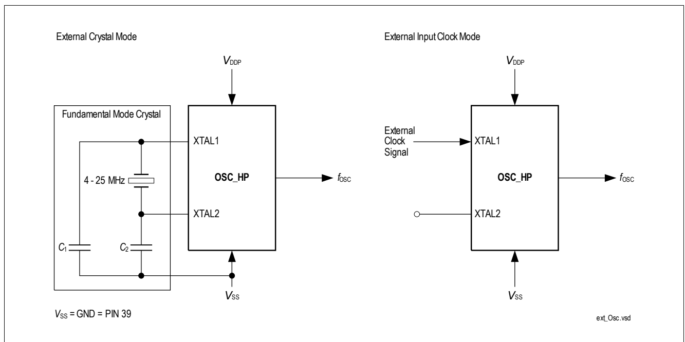
Figure 25 TLE987xQX External Circuitry for the OSC_HP
