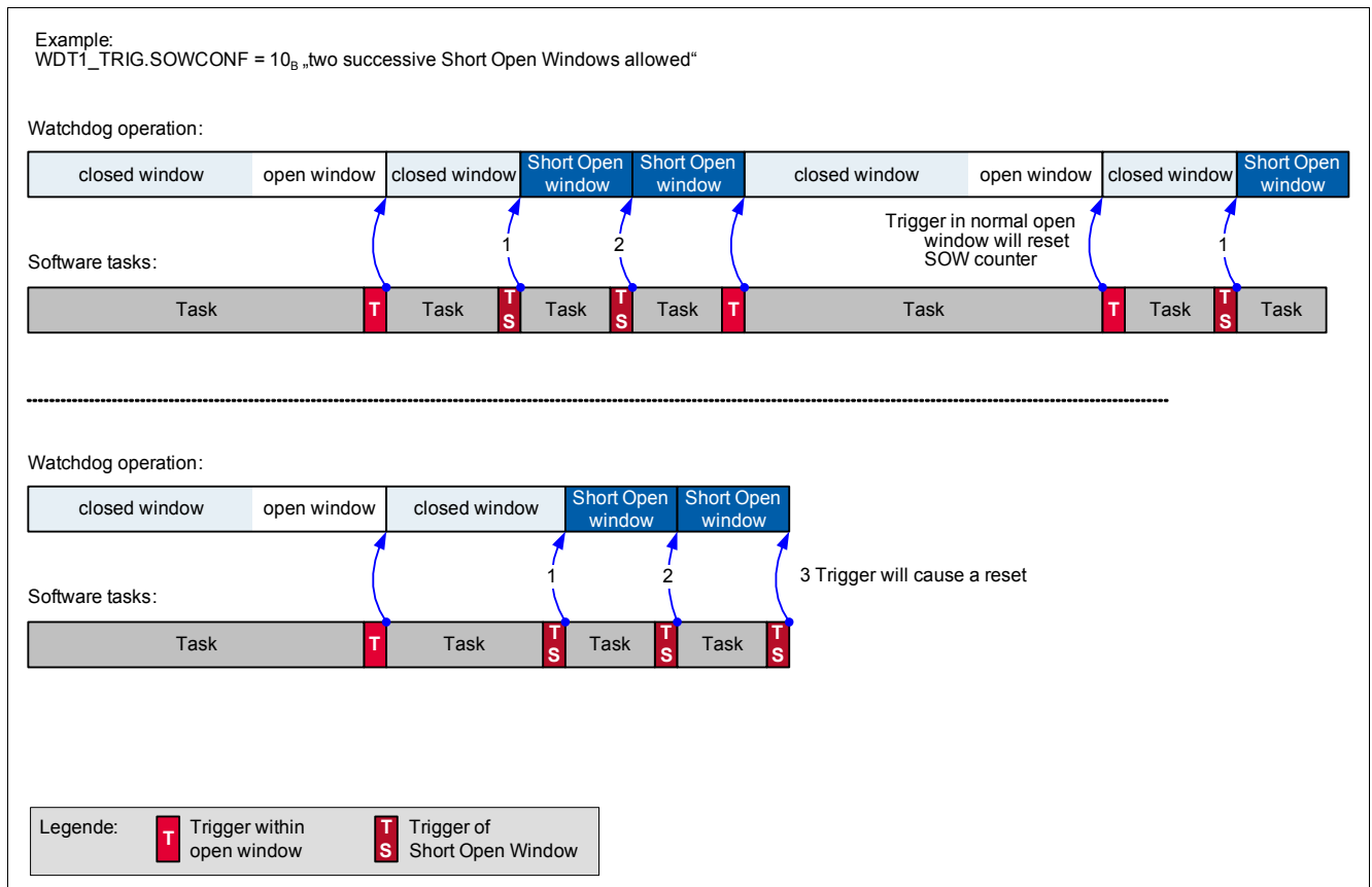
Figure 74 SOW Counter
