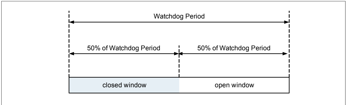
Figure 71 Windowed Watchdog
