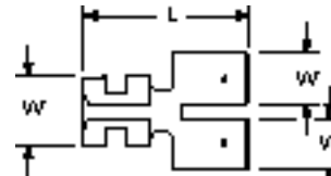
MA250DMMF 0.250 Male/Females (2)
