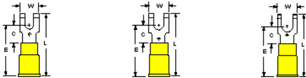
MV10-6FFBK MV10-8FFBK MV10-10FFBK Stud Size 6 8 10 Wire Range 12-10 12-10 12-10
