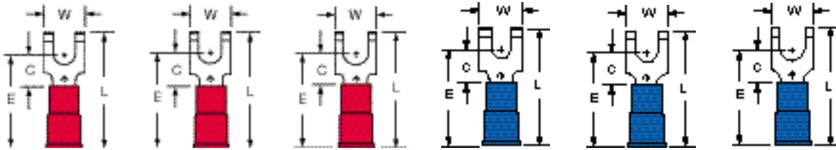
MV18-6FFBK MV18-8FFBK MV18-10FFBK MV14-6FFBK MV14-8FFBK MV14-10FFBK Stud Size 6 8 10 6 8 10 Wire Range 22-18 22-18 22-18 16-14 16-14 16-14
