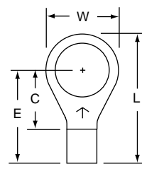
M10-516R/S Stud Size 5/16 Wire Range 12-10
