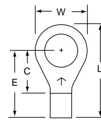
M10-38R/S Stud Size 3/8 Wire Range 12-10
