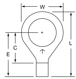
M10-12R Stud Size 1/2 Wire Range 12-10
