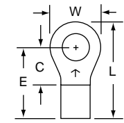
M10-10R Stud Size 10 Wire Range 12-10
