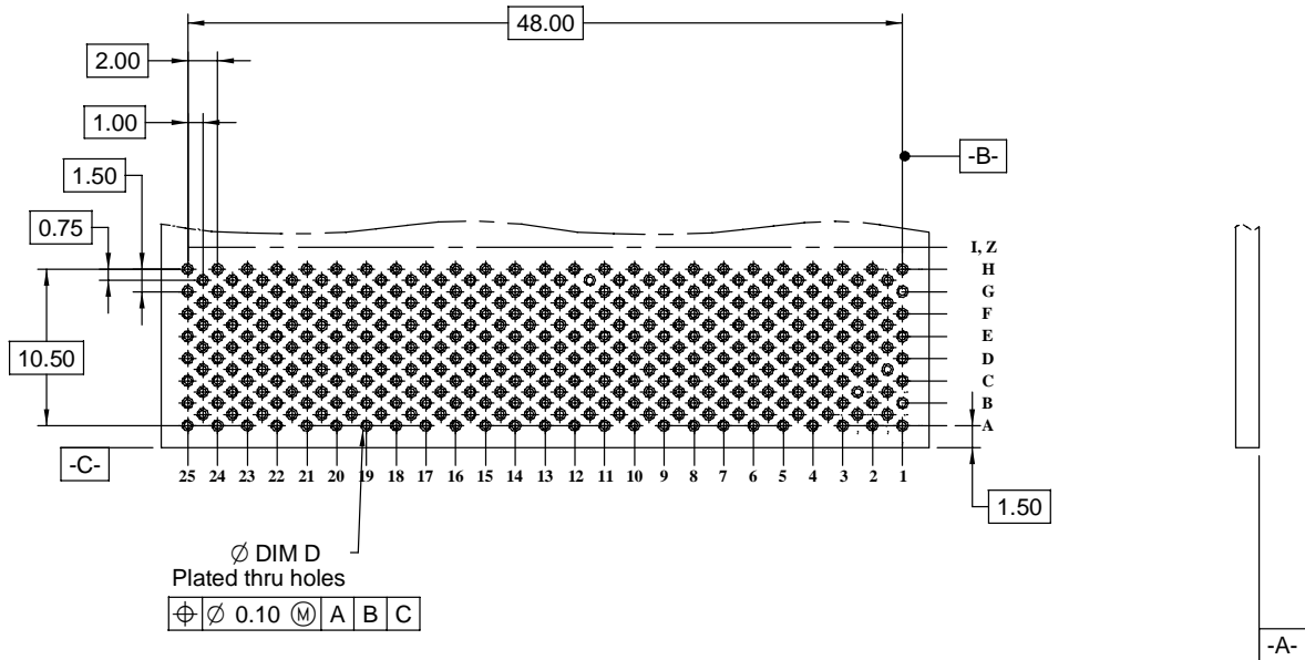
Recommended PCB hole mounting pattern for coaxial, column differential, and stripline applications
