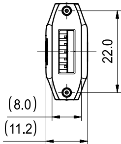
"SA2" WITH LOCKING SCREW
