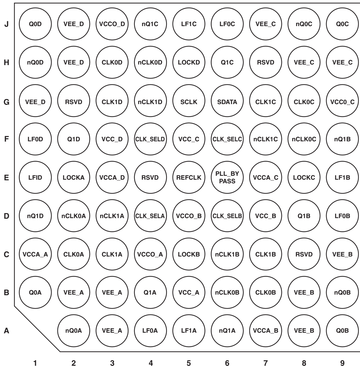
IDT8T49N488I Pin Map (bottom view)
