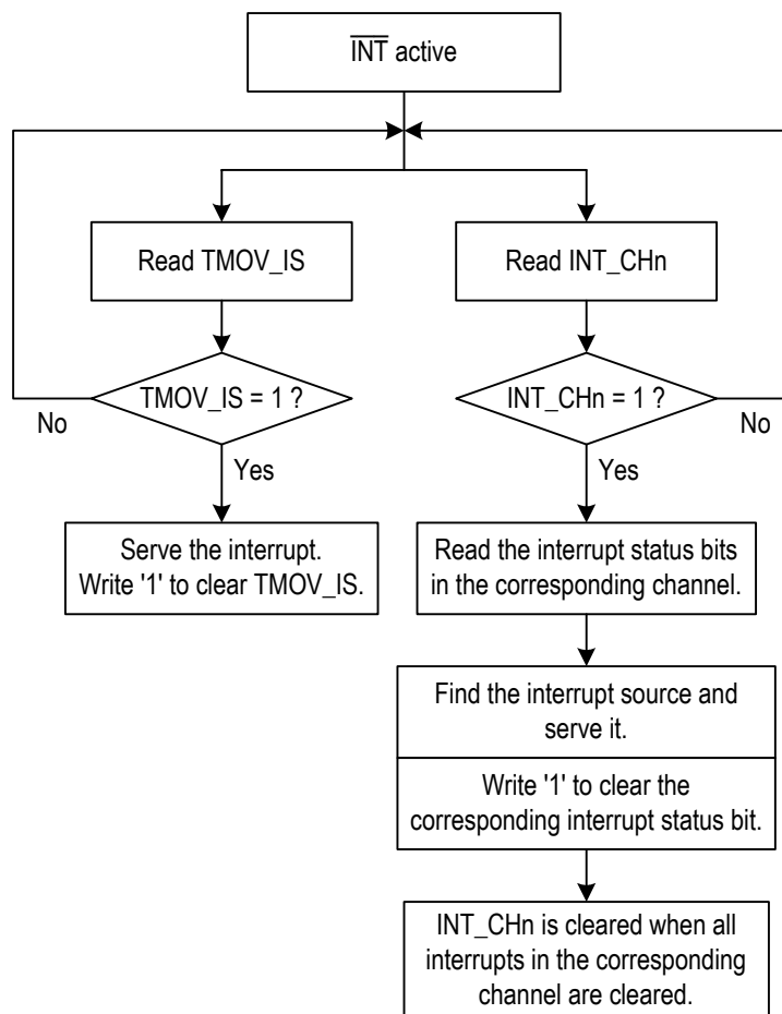
Figure-40 Interrupt Service Process
