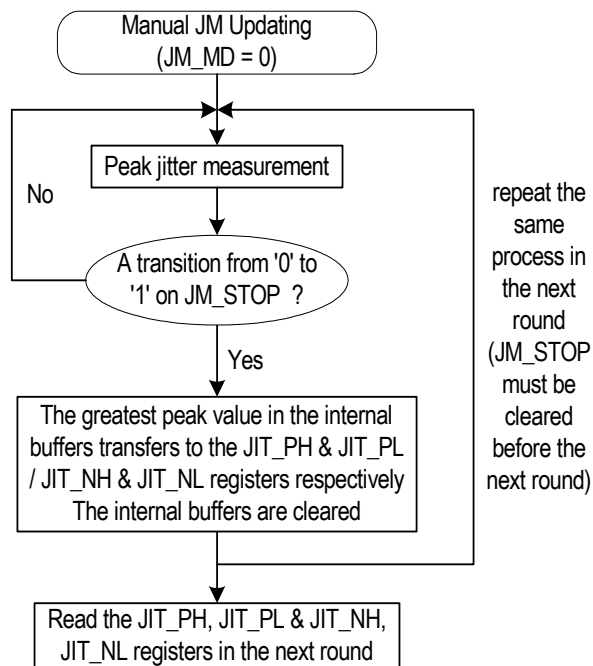
Figure-35 Manual JM Updating
