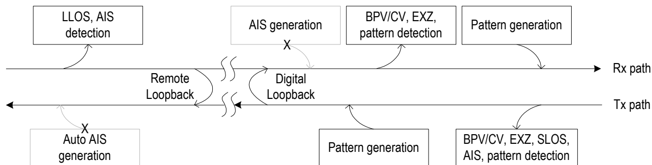
Figure-31 Priority Of Diagnostic Facilities During Manual Remote Loopback + Manual Digital Loopback
