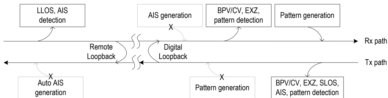
Figure-32 Priority Of Diagnostic Facilities During Manual Remote Loopback + Automatic Digital Loopback
