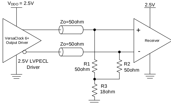
Figure 16. 2.5V LVPECL Output Termination (2)
