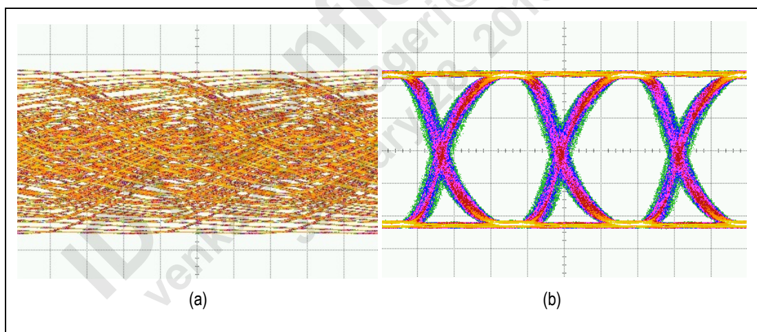
Figure 4 Eye Diagram
