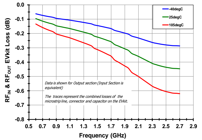
EVKit losses vs. Temperature
