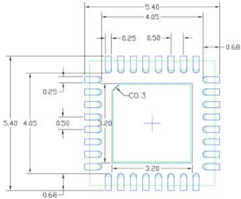
RECOMMENDED REDUCED LAND PATTERN DIMENSION
