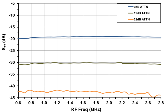
S 12 (device+C5 cap) [ T_{AMB} = 25C, V_{CC} = 5.00 Volts]
