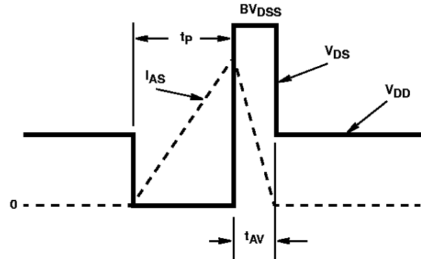
FIGURE 16. UNCLAMPED ENERGY WAVEFORM
