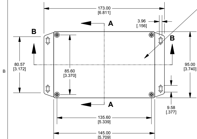
Top View of Assembly
