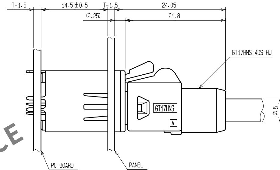
MATED CONNECTORS
