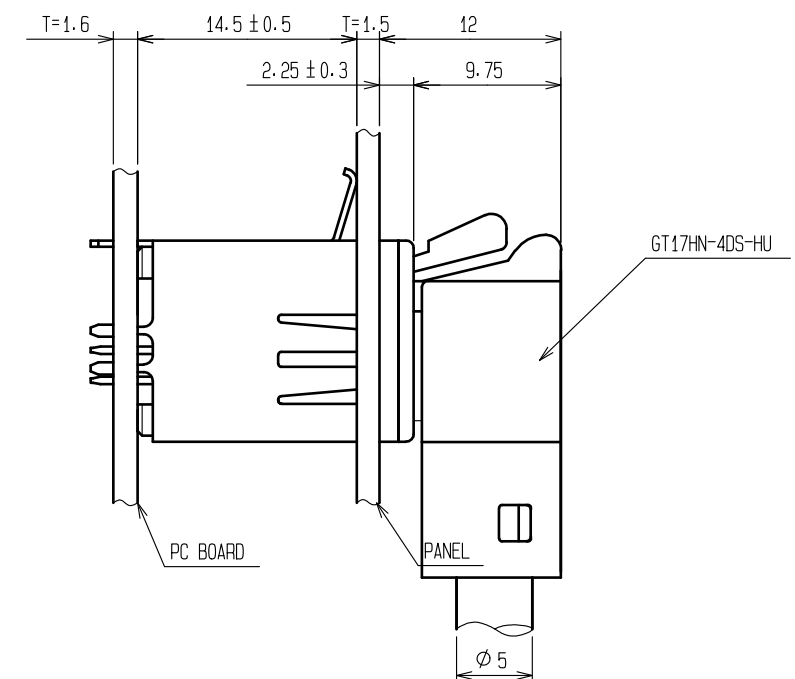
MATED CONNECTORS
