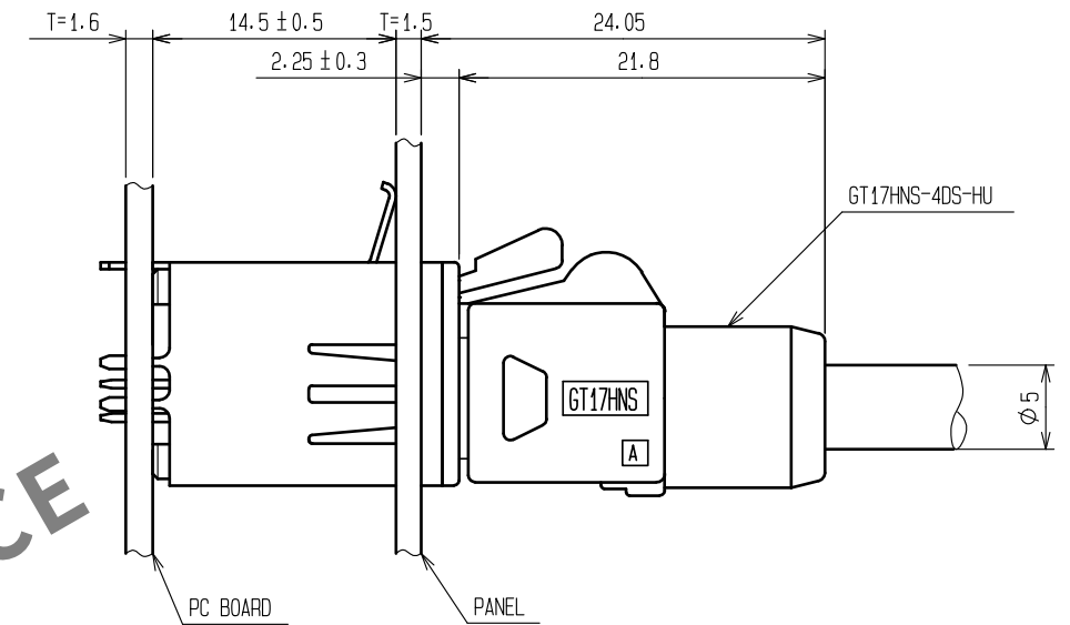
MATED CONNECTORS
