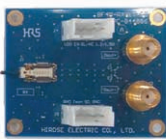
BF4M High Speed Transmission Board : RX2
