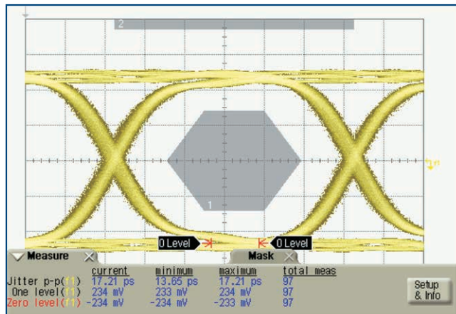
Eye Diagram (Typical) : Transmission Speed 6.25 Gbps, Length 5 meters
