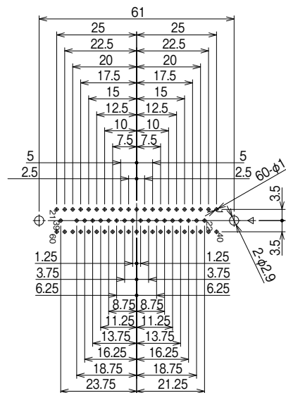
SD-1660A(10)
