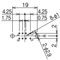
SD-1608A(09)
