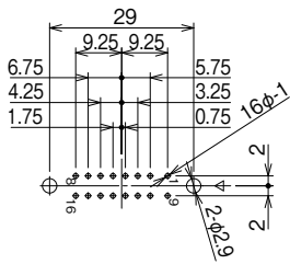
SD-1616A(09)
