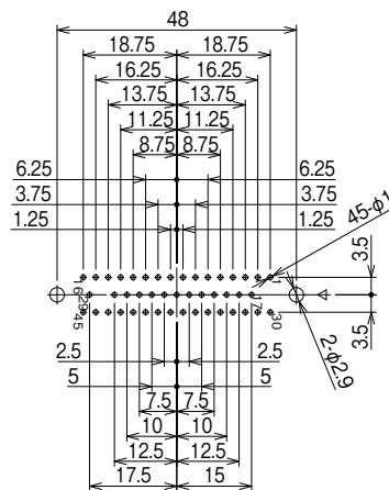
SD-1628A(09)
