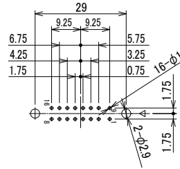
PD-1616BA(09)
