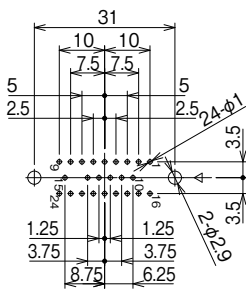
SD-1624A(09)
