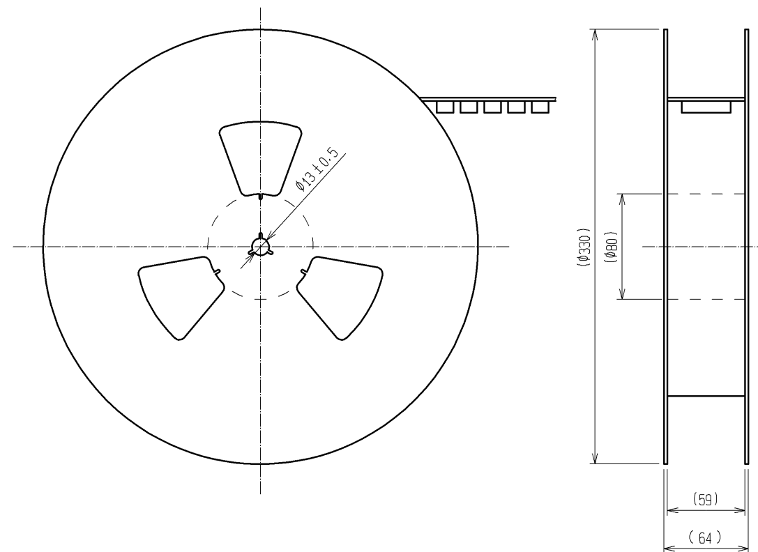
REELED DIMENSION(Free)
