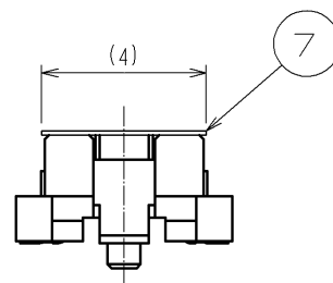
DETAIL FOR VACUUM PICKUP (5:1)
